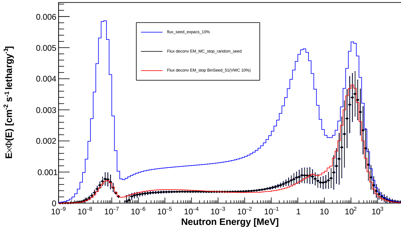
Spectrum_LCO_Event_133_timegrid_15_ndet_11_Random_Seed
