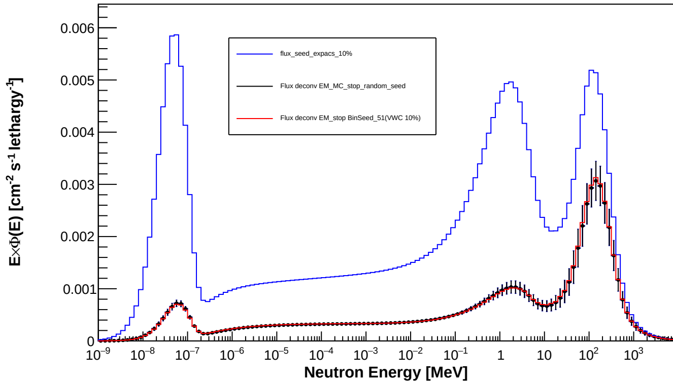
Spectrum_LCO_Event_135_timegrid_15_ndet_11_Random_Seed
