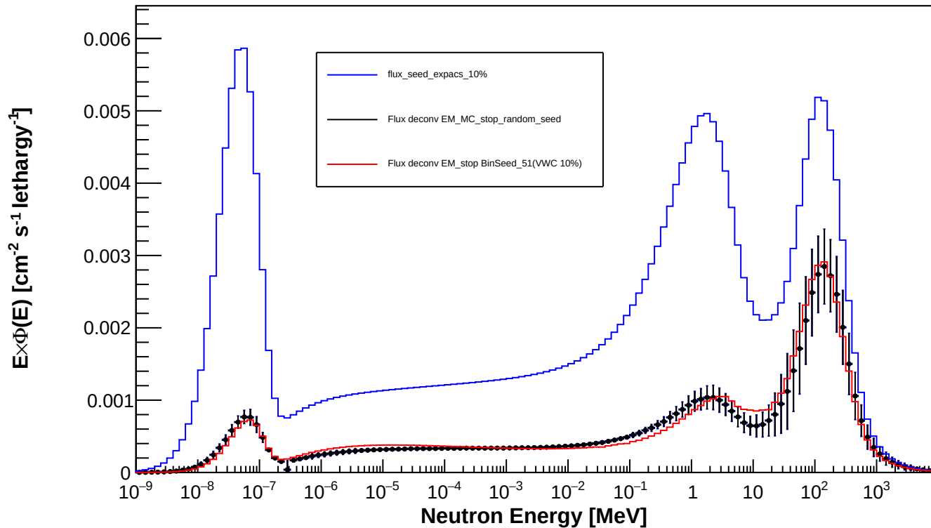
Spectrum_LCO_Event_138_timegrid_15_ndet_11_Random_Seed
