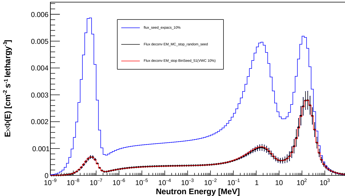
Spectrum_LCO_Event_145_timegrid_15_ndet_11_Random_Seed
