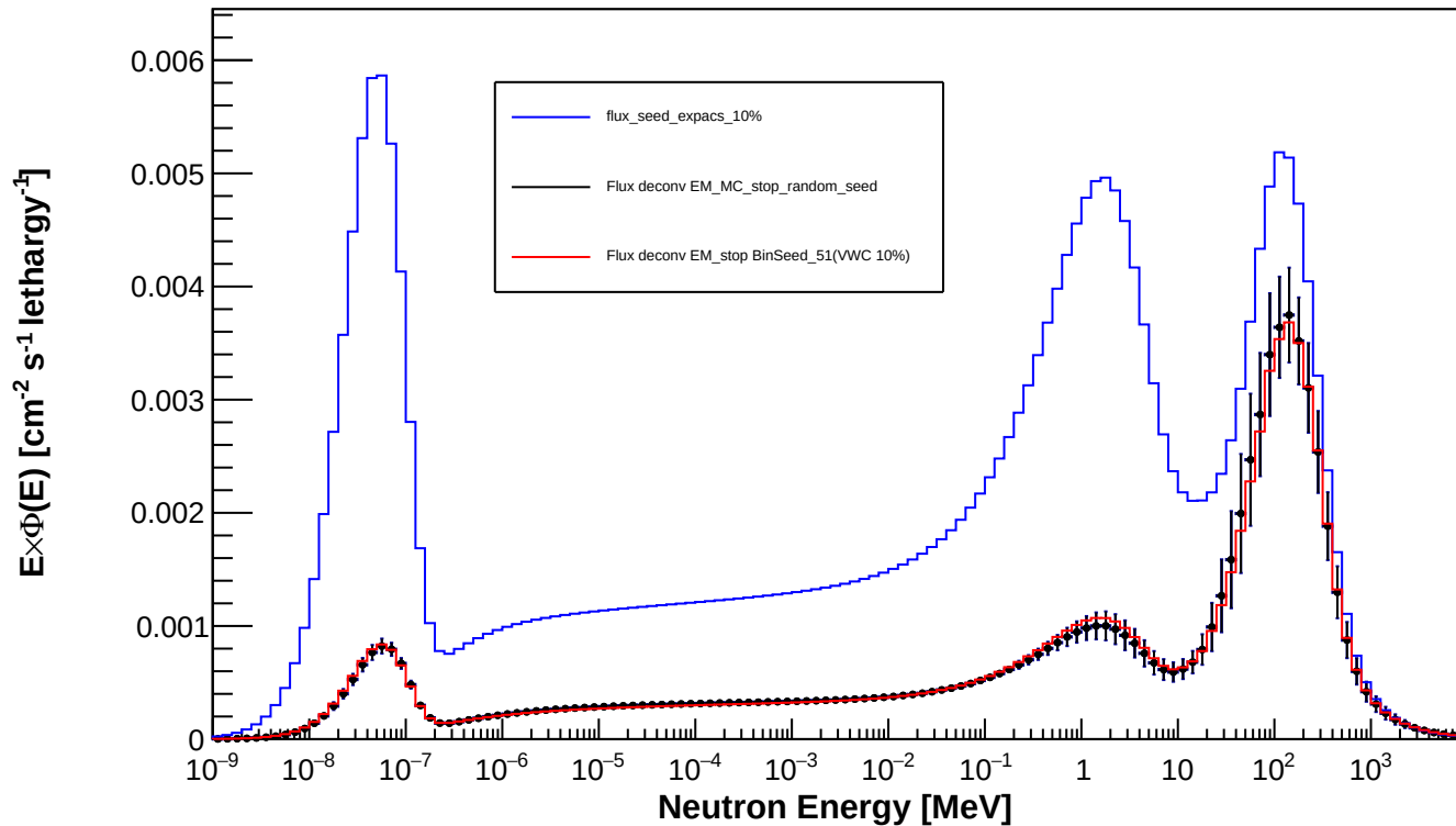
Spectrum_LCO_Event_148_timegrid_15_ndet_11_Random_Seed
