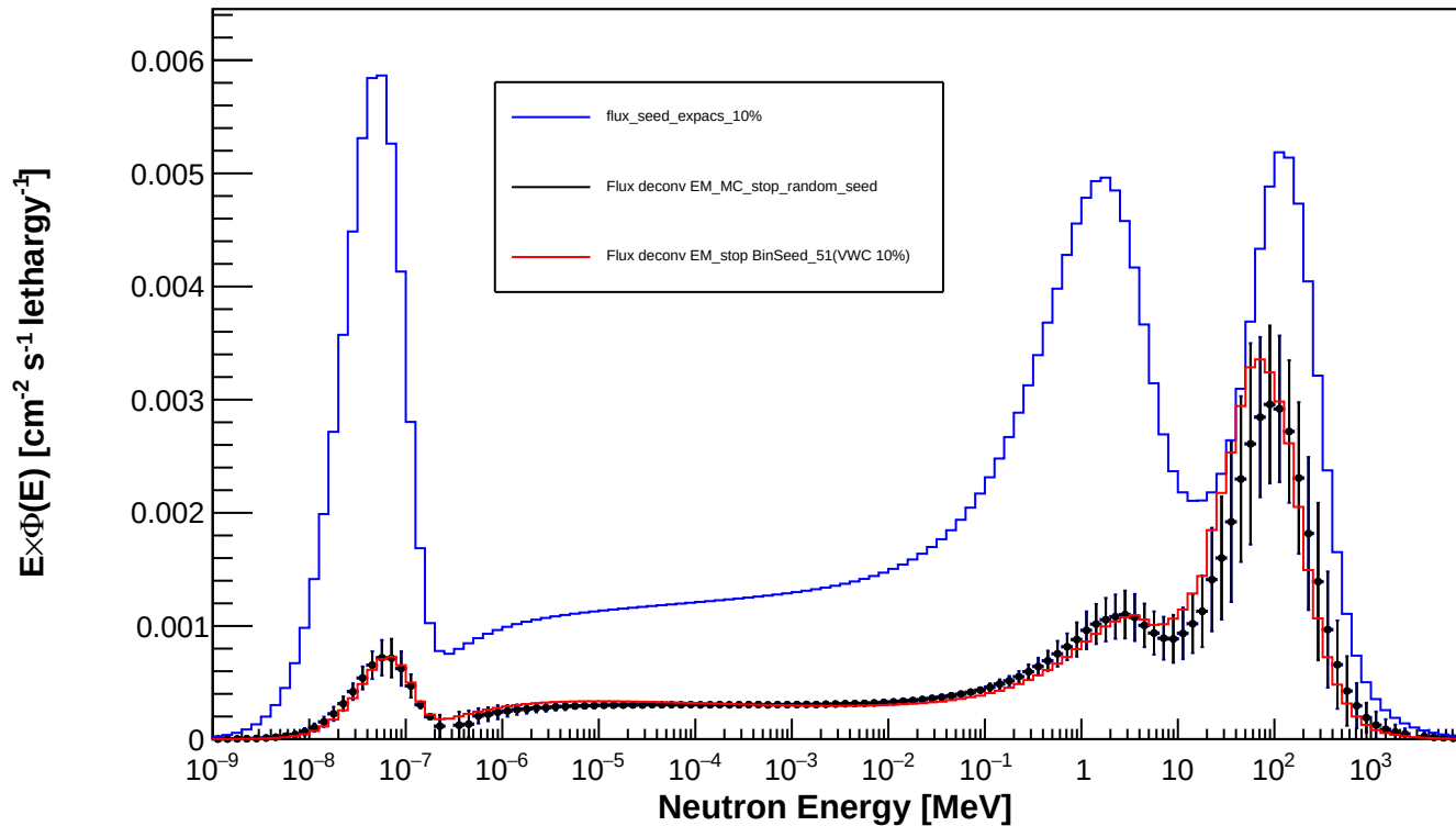
Spectrum_LCO_Event_149_timegrid_15_ndet_11_Random_Seed
