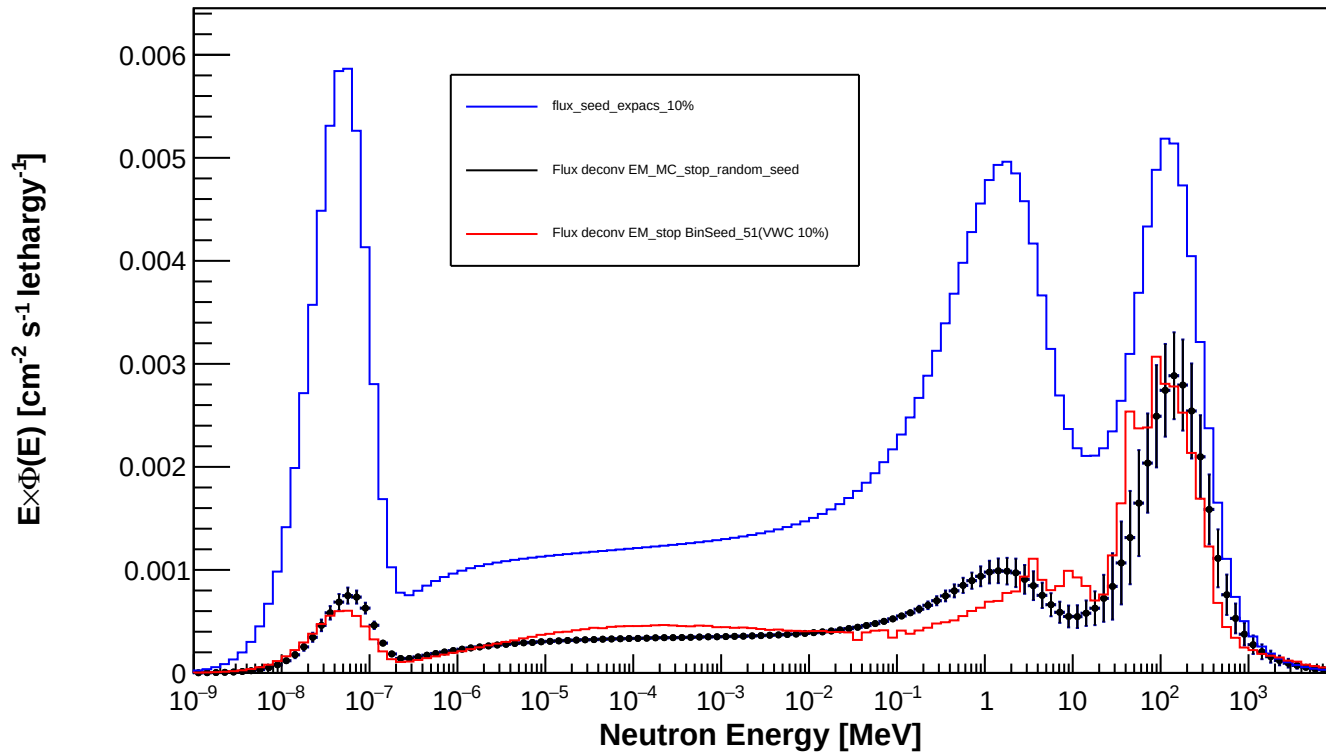
Spectrum_LCO_Event_153_timegrid_15_ndet_11_Random_Seed
