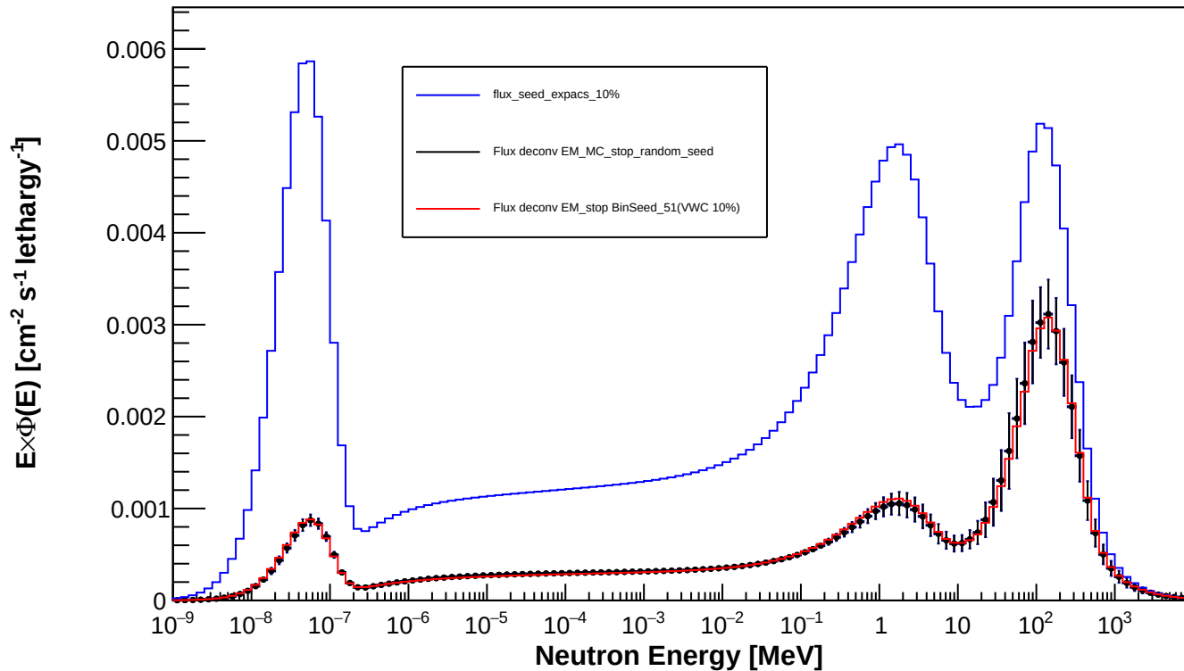
Spectrum_LCO_Event_157_timegrid_15_ndet_11_Random_Seed
