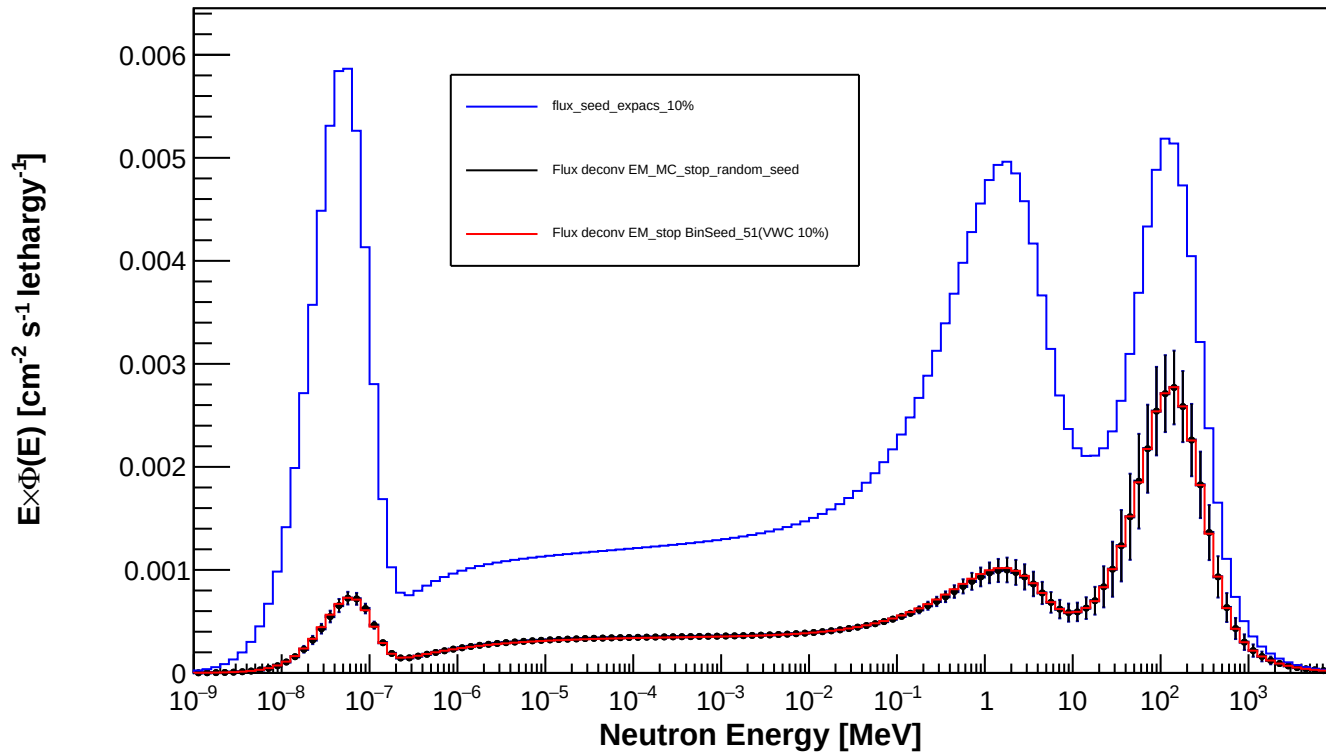
Spectrum_LCO_Event_162_timegrid_15_ndet_11_Random_Seed
