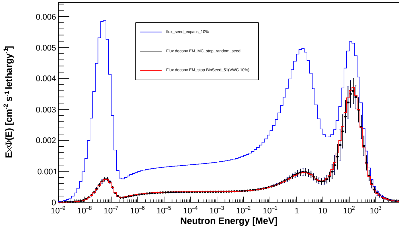
Spectrum_LCO_Event_170_timegrid_15_ndet_11_Random_Seed
