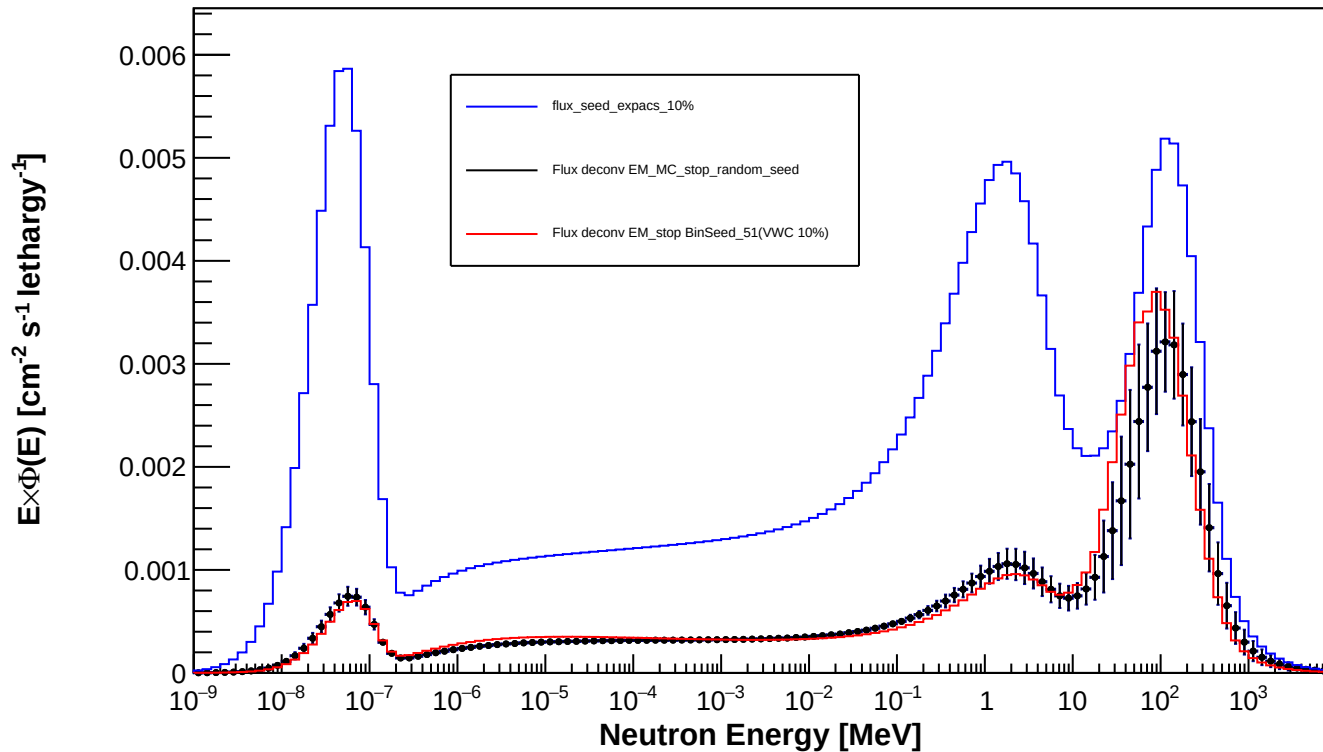
Spectrum_LCO_Event_182_timegrid_15_ndet_11_Random_Seed
