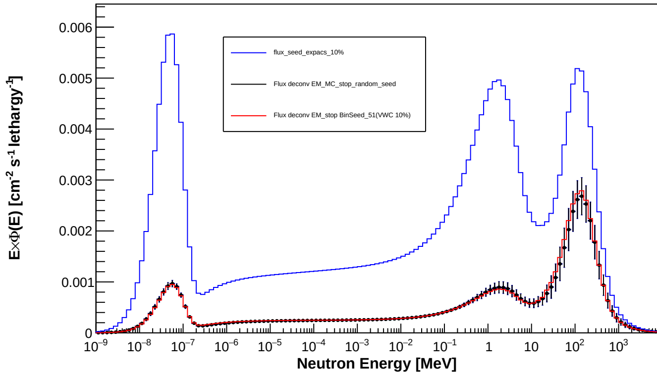
Spectrum_LCO_Event_198_timegrid_15_ndet_11_Random_Seed
