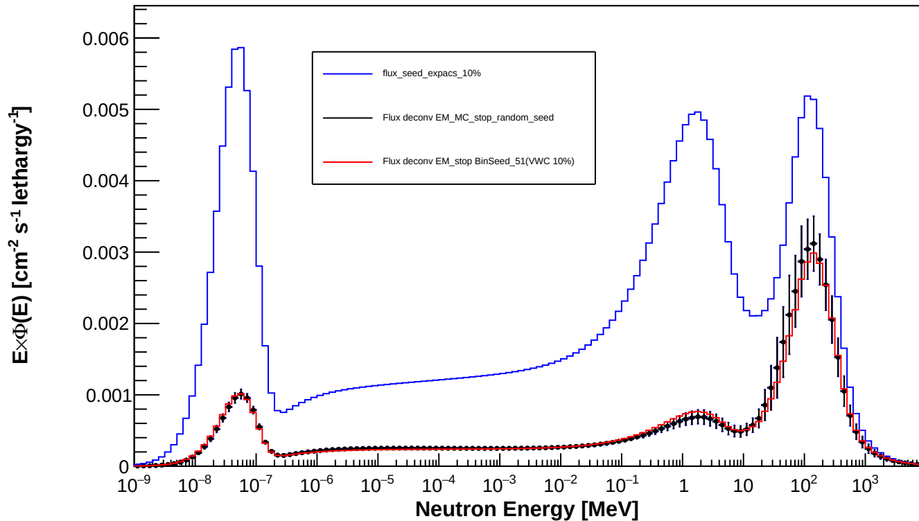
Spectrum_LCO_Event_211_timegrid_15_ndet_11_Random_Seed
