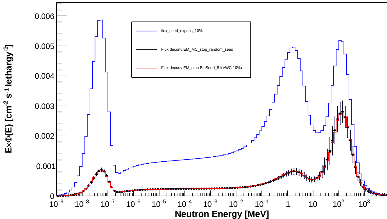
Spectrum_LCO_Event_221_timegrid_15_ndet_11_Random_Seed
