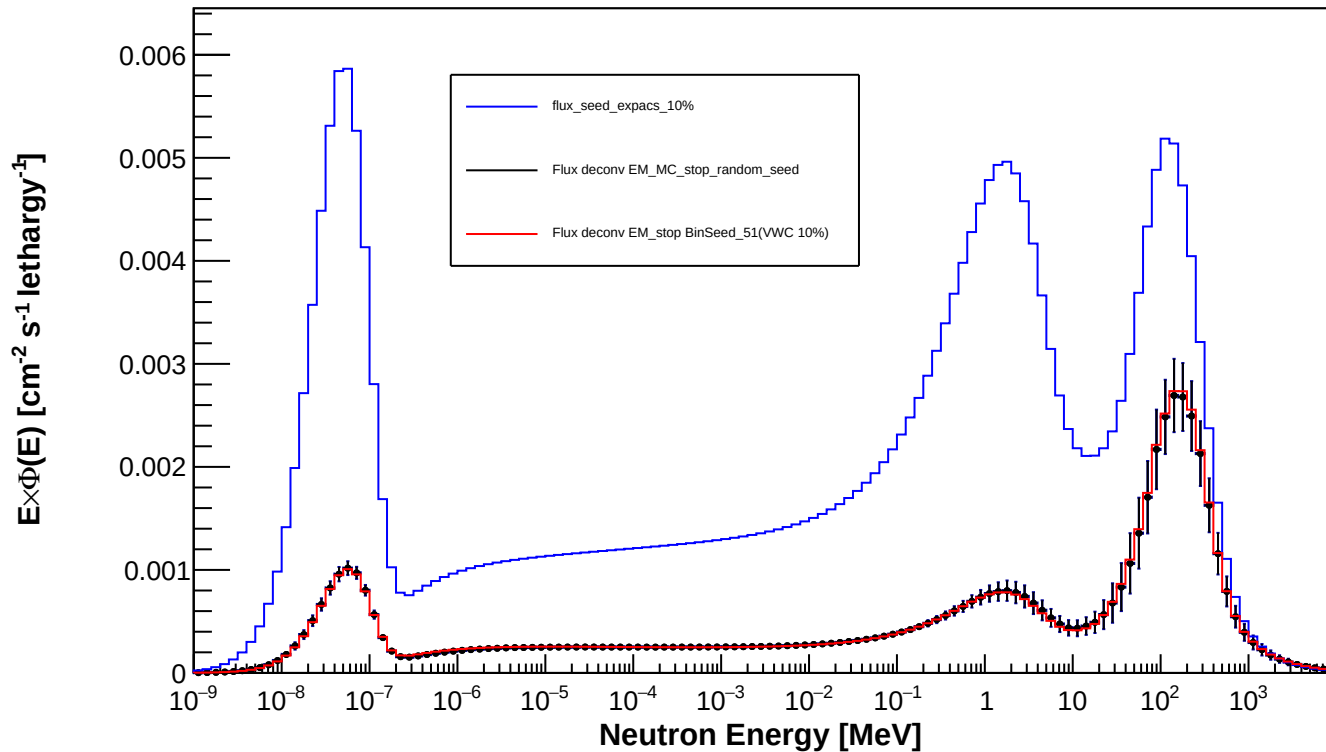
Spectrum_LCO_Event_226_timegrid_15_ndet_11_Random_Seed
