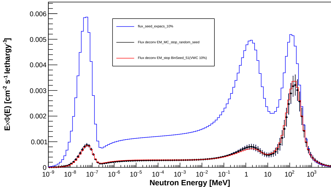
Spectrum_LCO_Event_231_timegrid_15_ndet_11_Random_Seed
