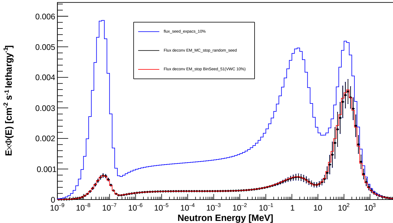
Spectrum_LCO_Event_248_timegrid_15_ndet_11_Random_Seed
