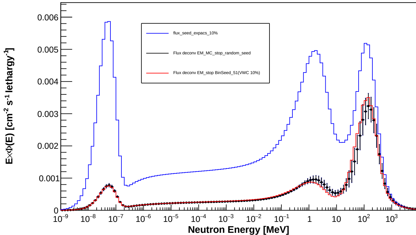
Spectrum_LCO_Event_251_timegrid_15_ndet_11_Random_Seed
