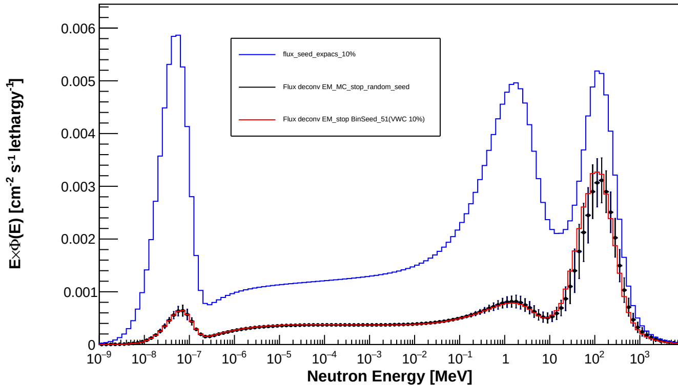
Spectrum_LCO_Event_25_timegrid_15_ndet_11_Random_Seed
