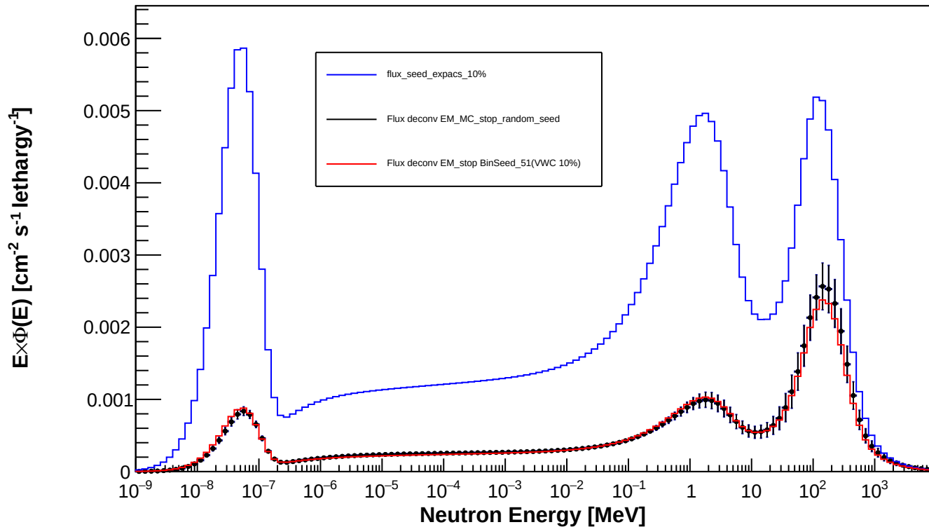
Spectrum_LCO_Event_285_timegrid_15_ndet_11_Random_Seed
