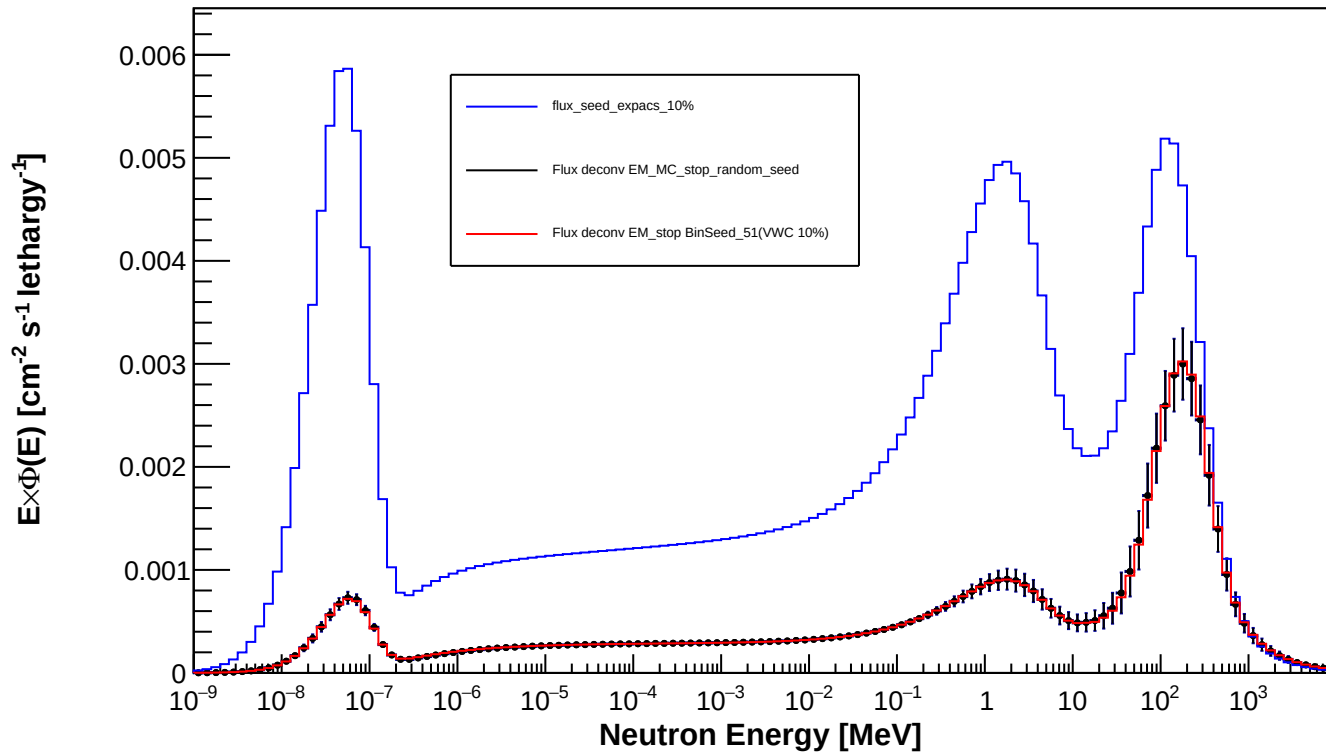
Spectrum_LCO_Event_289_timegrid_15_ndet_11_Random_Seed
