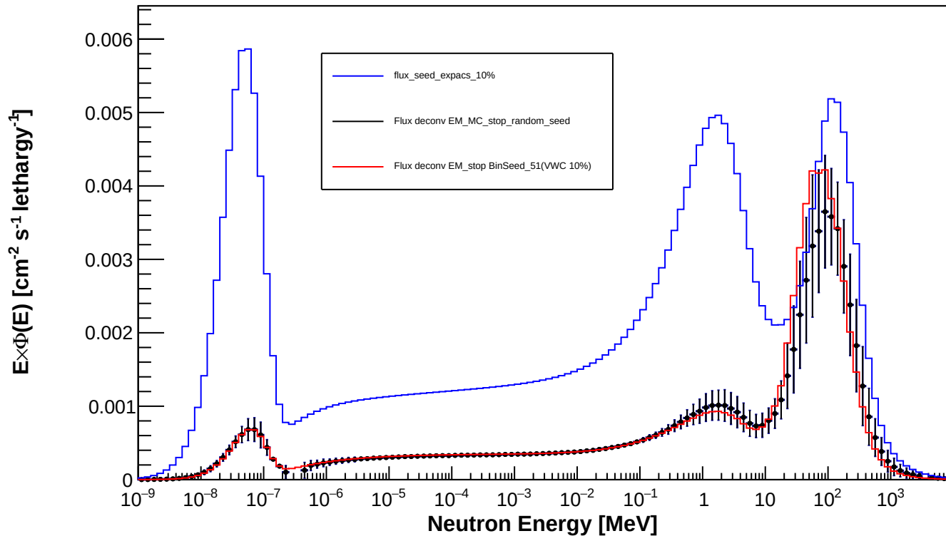
Spectrum_LCO_Event_51_timegrid_15_ndet_11_Random_Seed
