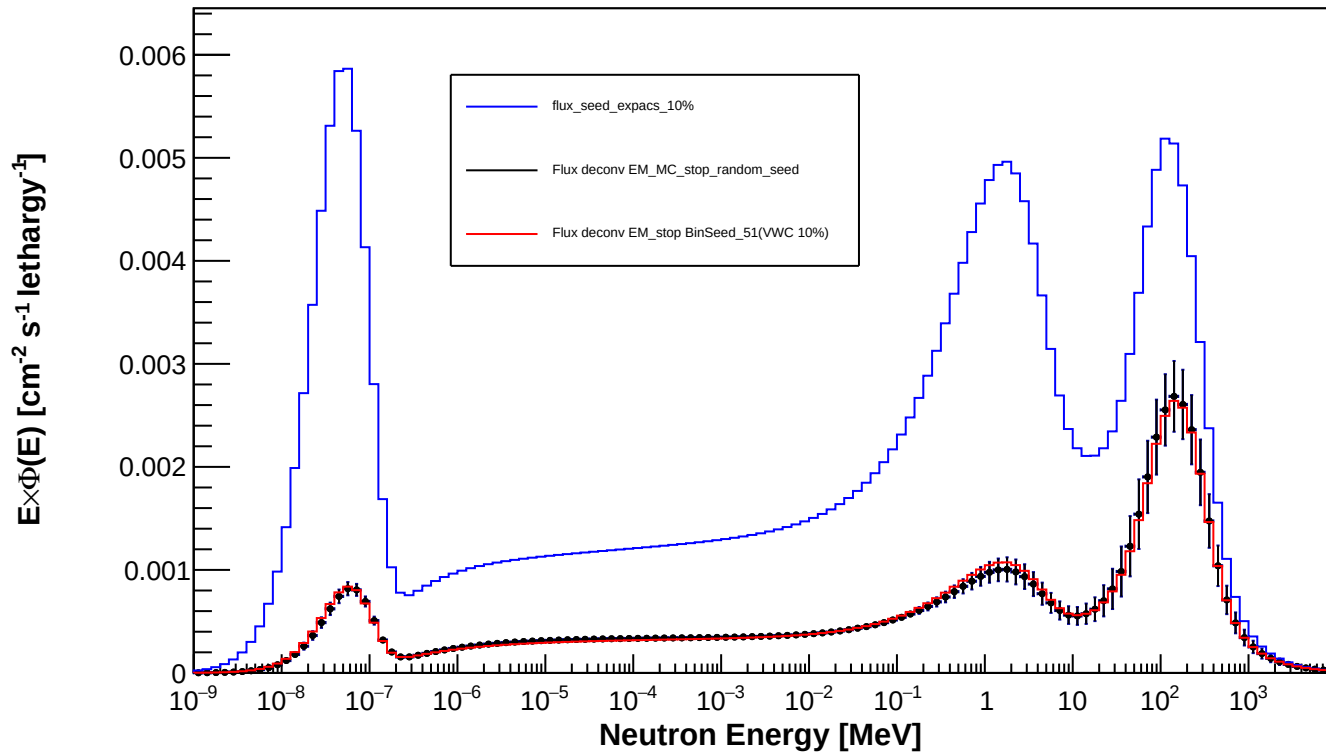
Spectrum_LCO_Event_52_timegrid_15_ndet_11_Random_Seed
