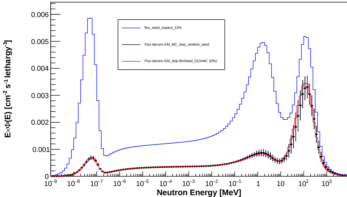
Spectrum_LCO_Event_53_timegrid_15_ndet_11_Random_Seed
