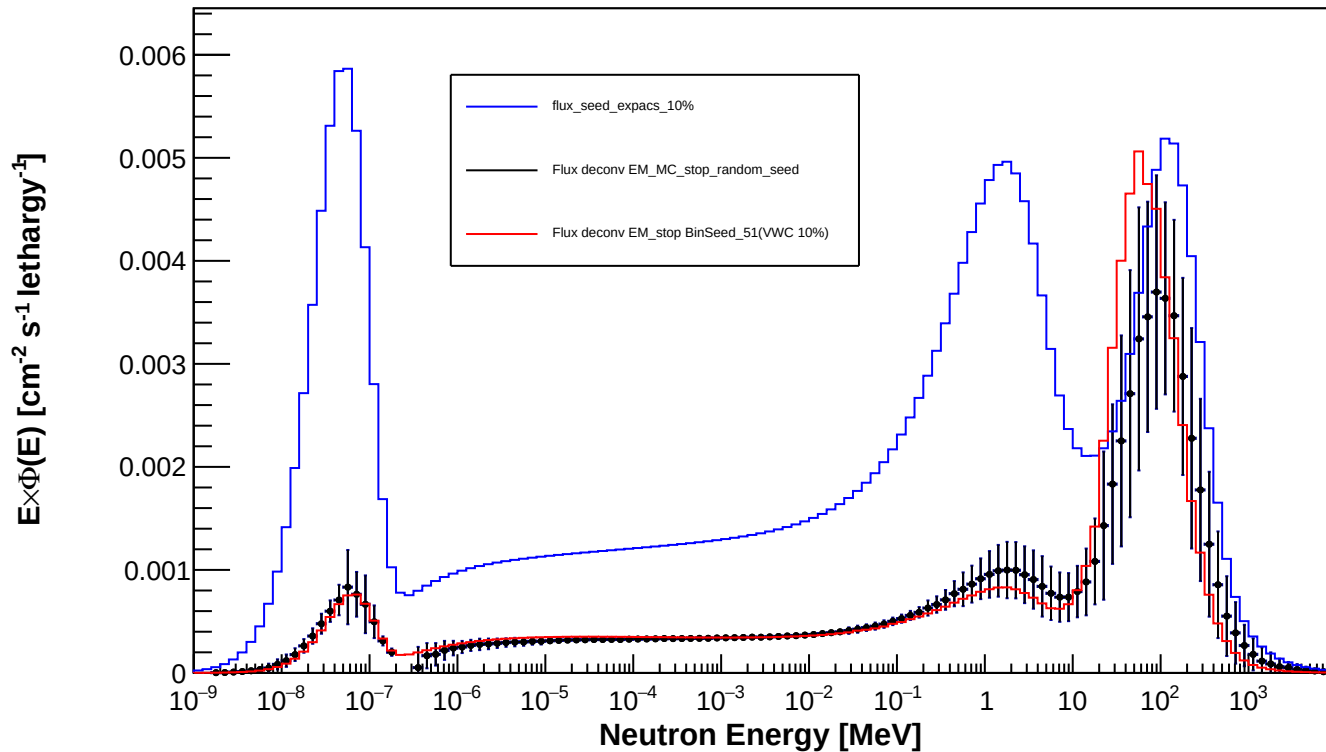
Spectrum_LCO_Event_64_timegrid_15_ndet_11_Random_Seed
