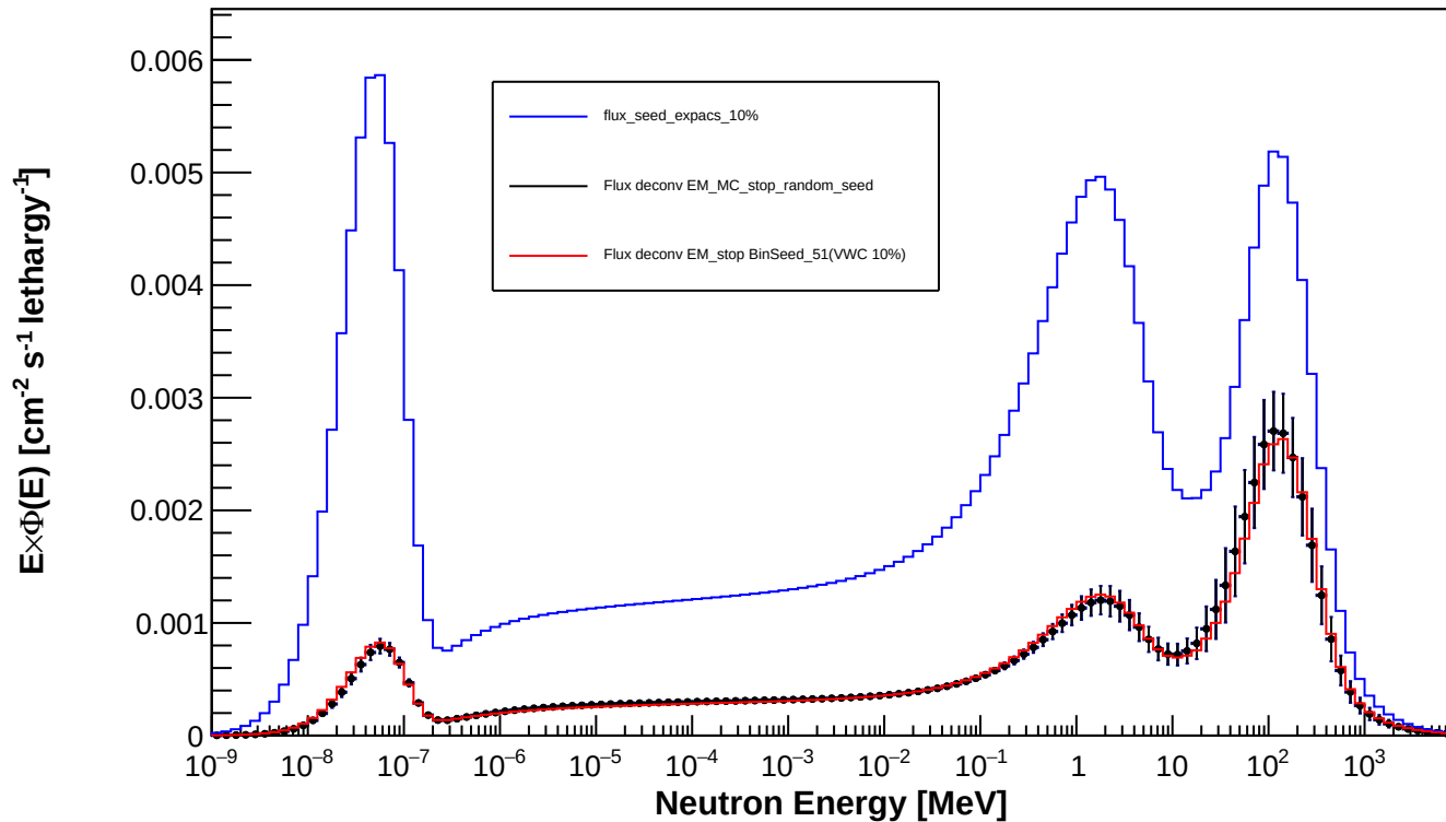
Spectrum_LCO_Event_76_timegrid_15_ndet_11_Random_Seed
