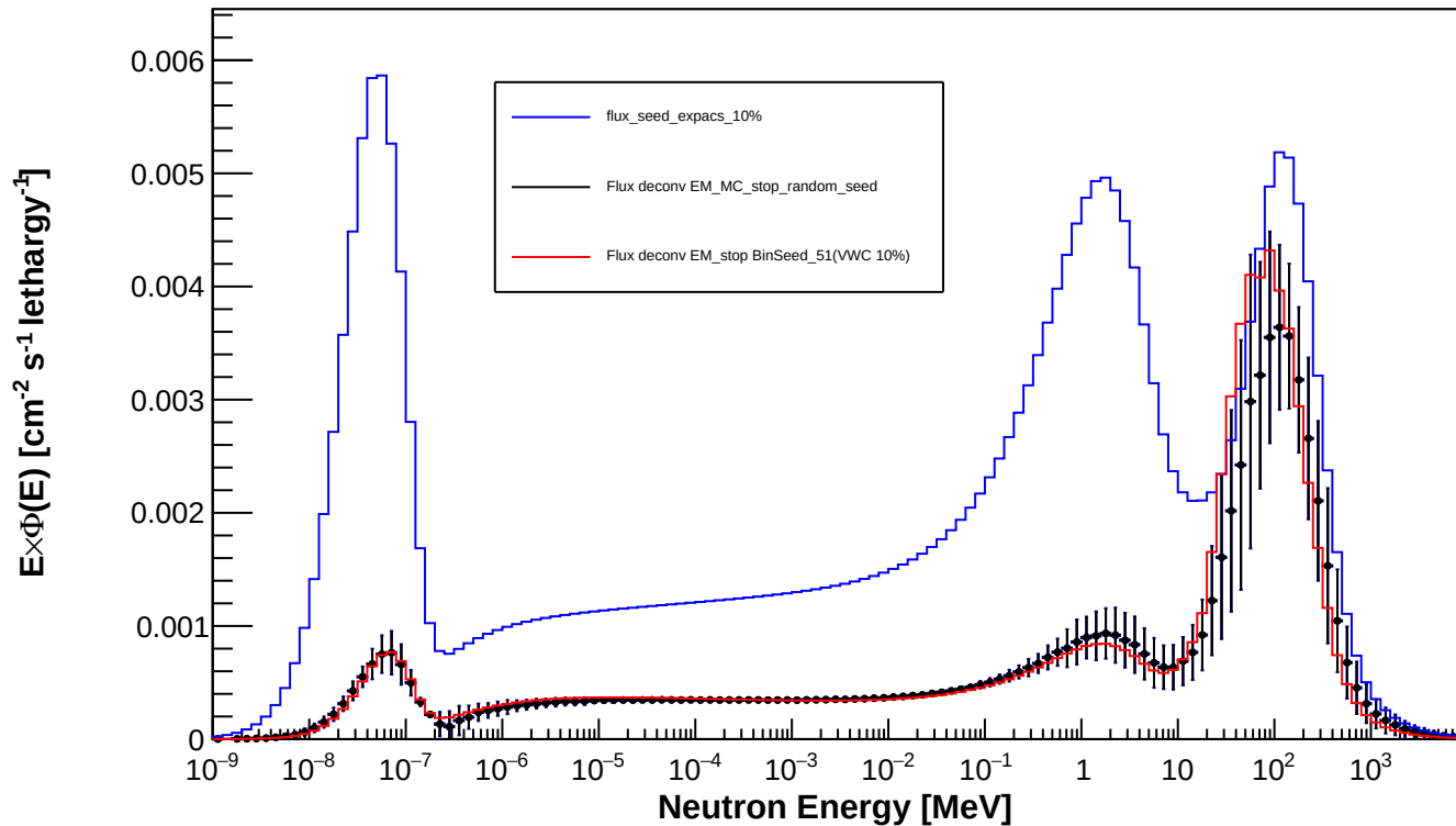
Spectrum_LCO_Event_77_timegrid_15_ndet_11_Random_Seed
