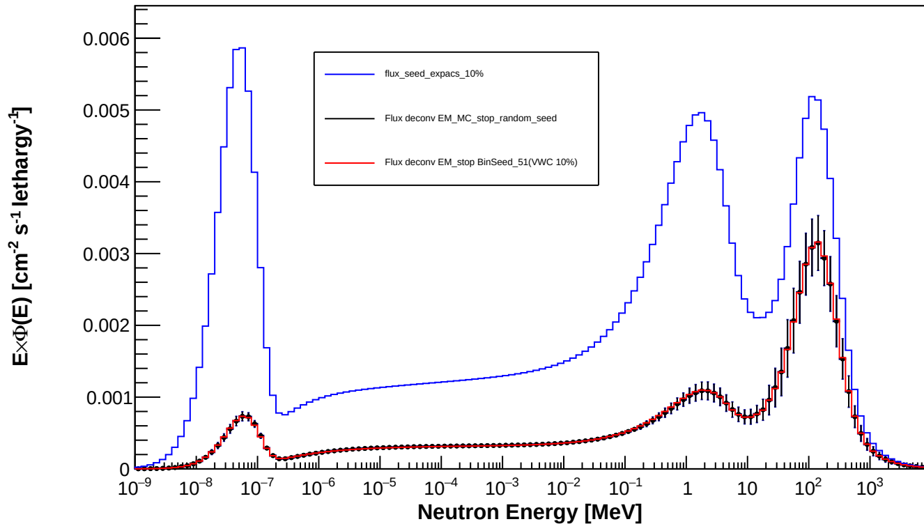
Spectrum_LCO_Event_79_timegrid_15_ndet_11_Random_Seed
