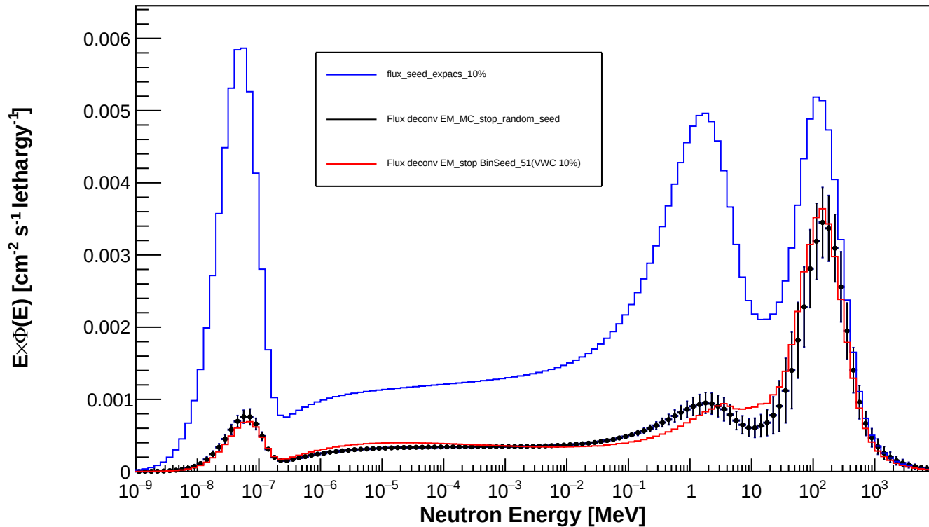
Spectrum_LCO_Event_14_timegrid_15_ndet_11_Random_Seed
