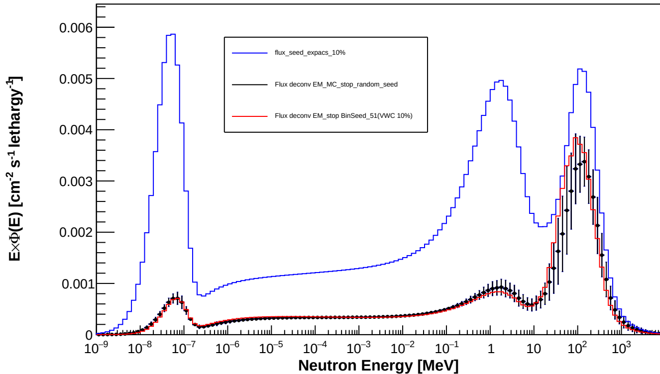
Spectrum_LCO_Event_11_timegrid_15_ndet_11_Random_Seed
