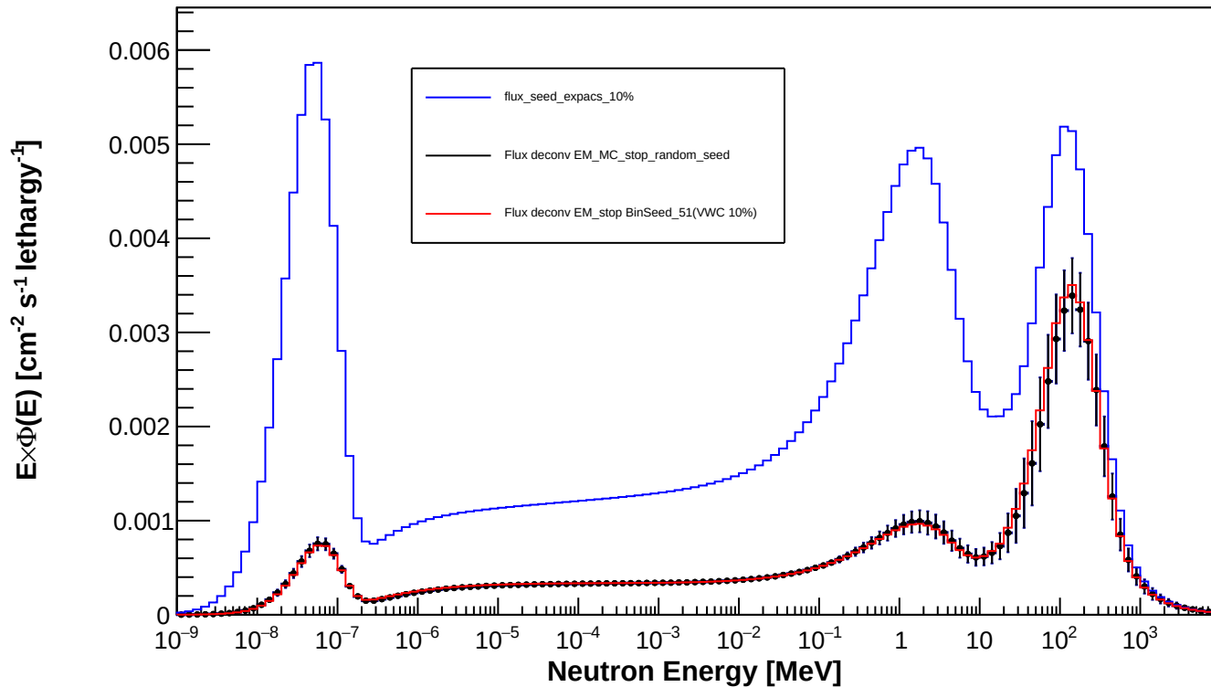
Spectrum_LCO_Event_6_timegrid_15_ndet_11_Random_Seed
