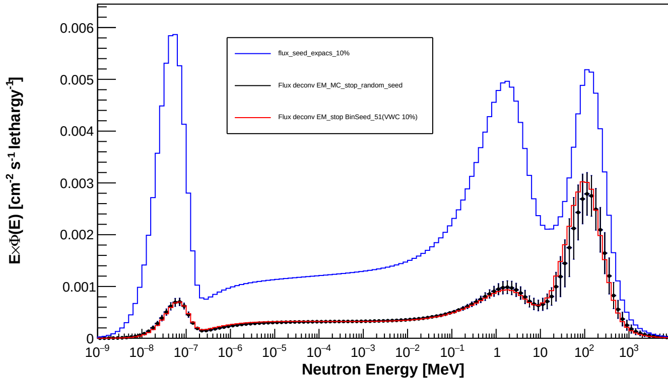
Spectrum_LCO_Event_10_timegrid_15_ndet_11_Random_Seed
