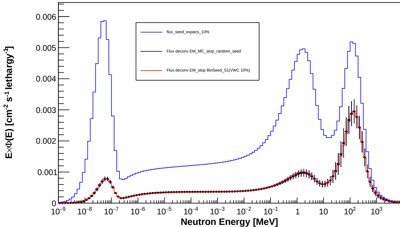
Spectrum_LCO_Event_3_timegrid_15_ndet_11_Random_Seed
