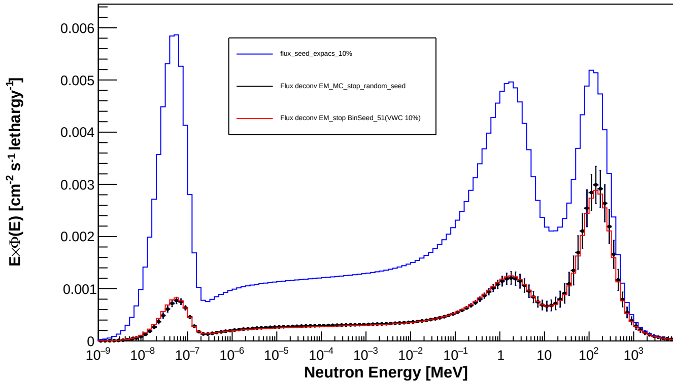
Spectrum_LCO_Event_2_timegrid_15_ndet_11_Random_Seed
