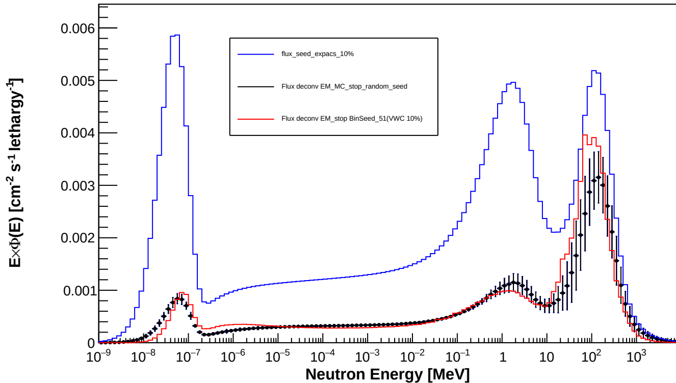
Spectrum_LCO_Event_16_timegrid_15_ndet_11_Random_Seed
