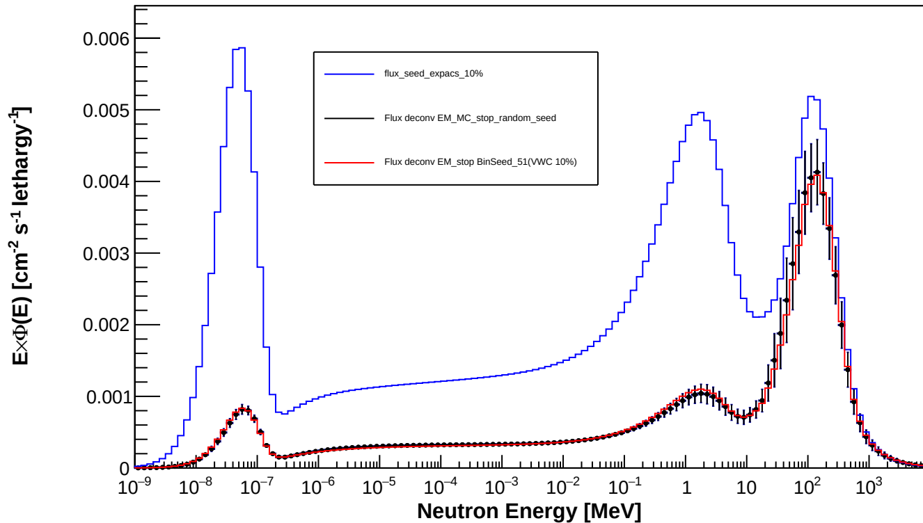
Spectrum_LCO_Event_17_timegrid_15_ndet_11_Random_Seed
