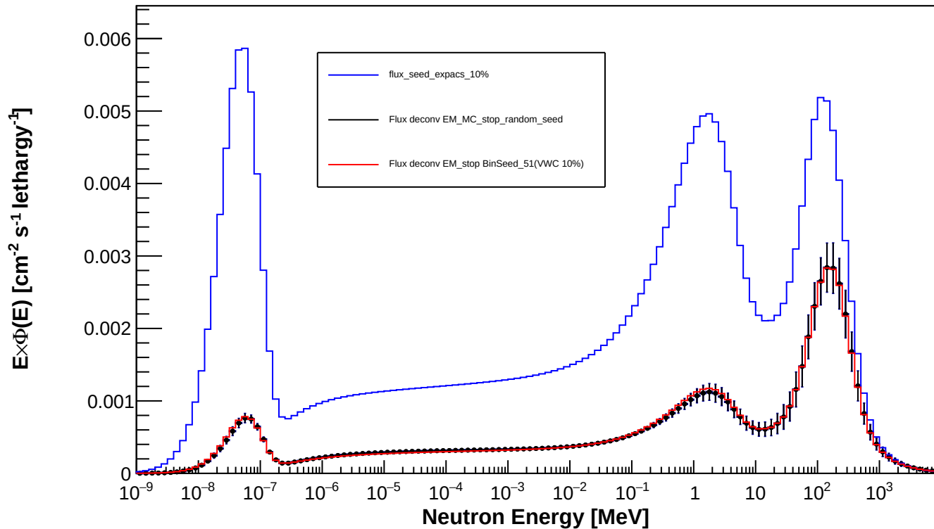
Spectrum_LCO_Event_7_timegrid_15_ndet_11_Random_Seed
