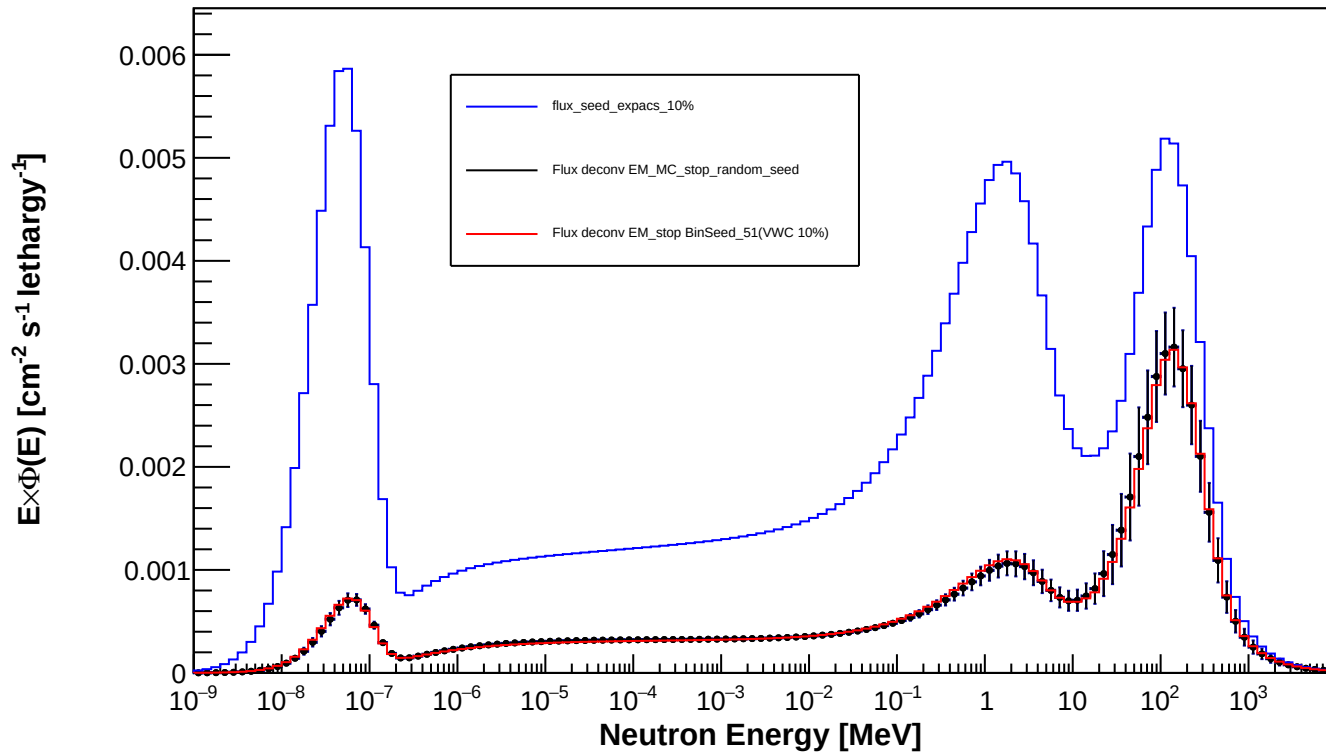
Spectrum_LCO_Event_19_timegrid_15_ndet_11_Random_Seed
