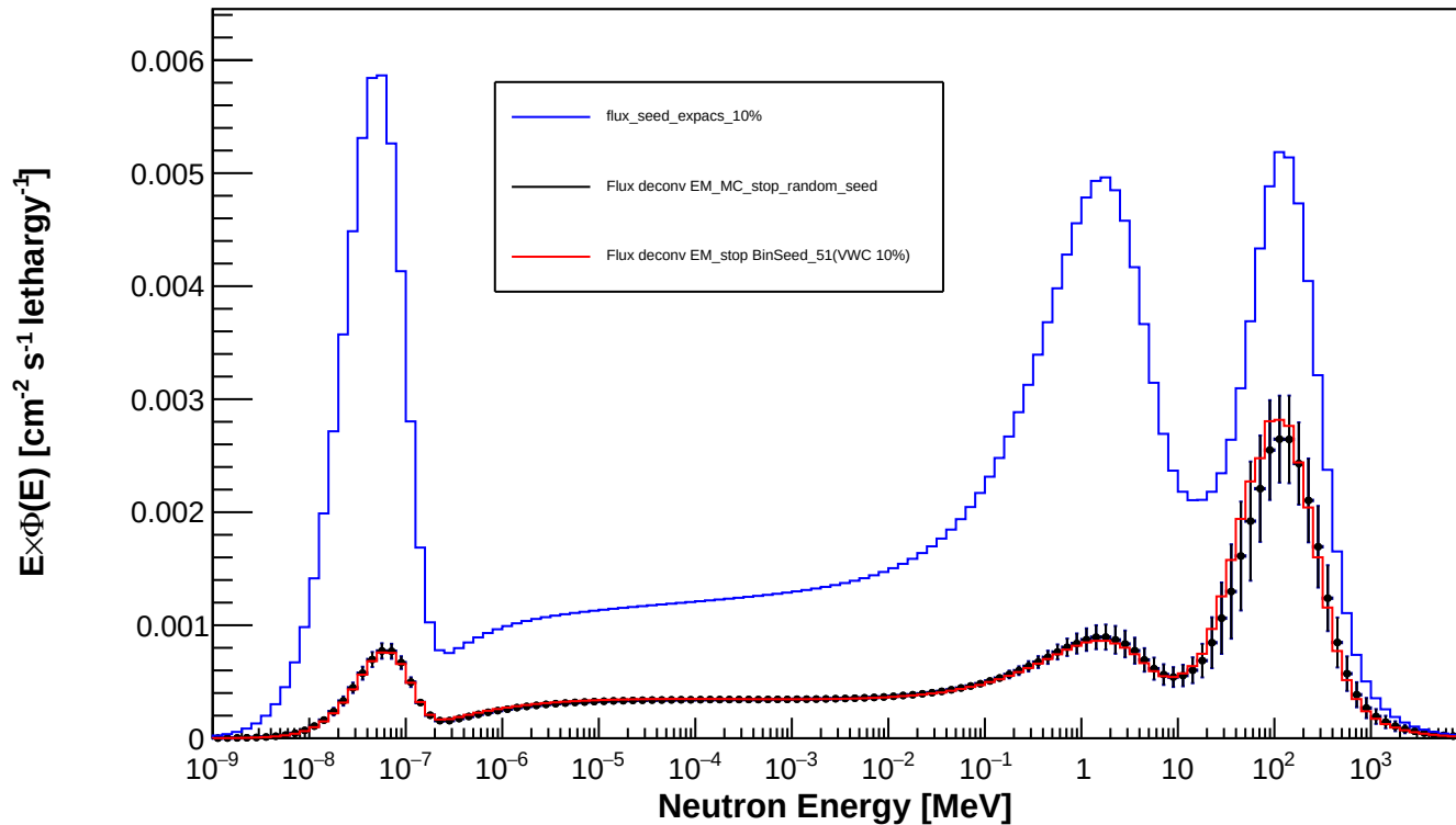
Spectrum_LCO_Event_4_timegrid_15_ndet_11_Random_Seed
