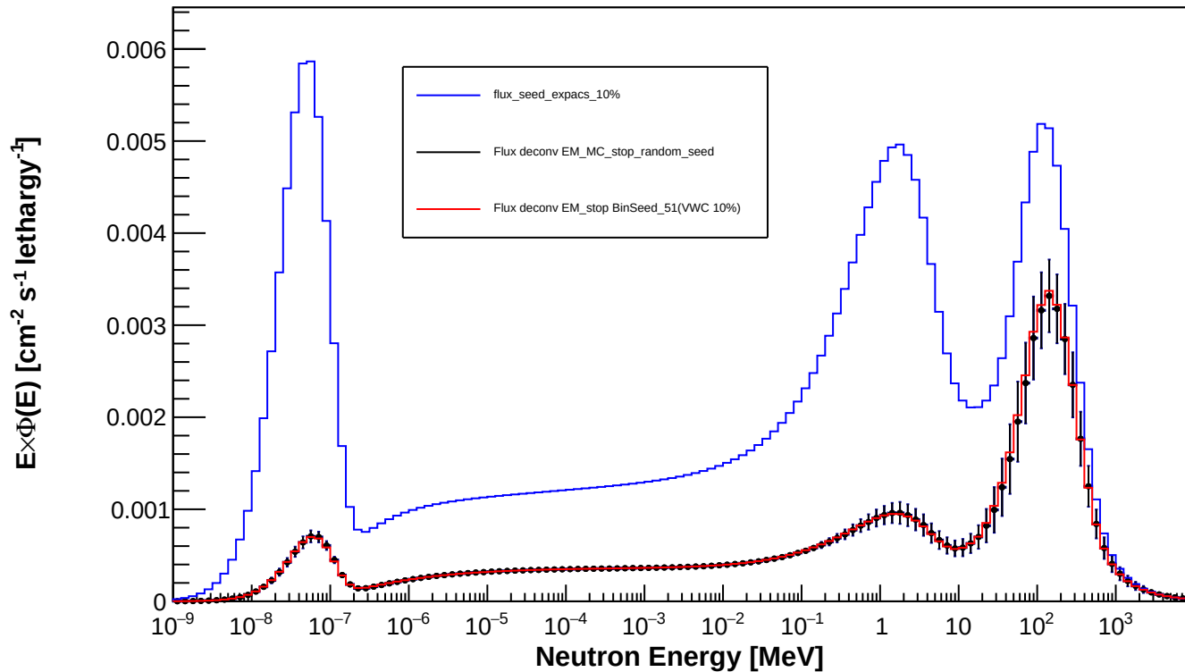
Spectrum_LCO_Event_5_timegrid_15_ndet_11_Random_Seed
