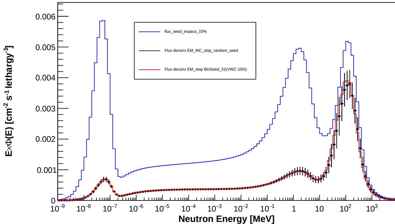
Spectrum_LCO_Event_18_timegrid_15_ndet_11_Random_Seed
