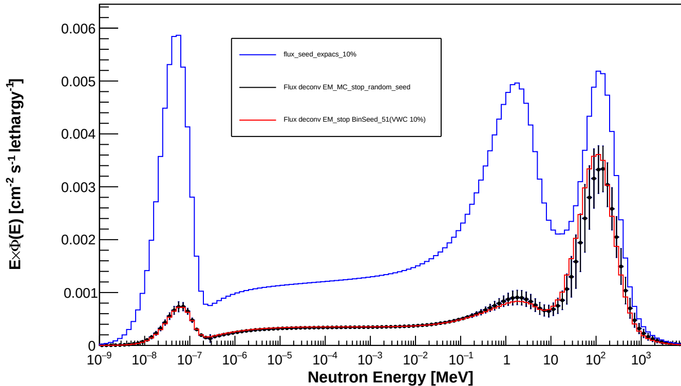
Spectrum_LCO_Event_9_timegrid_15_ndet_11_Random_Seed
