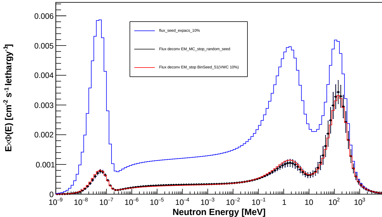
Spectrum_LCO_Event_21_timegrid_15_ndet_11_Random_Seed
