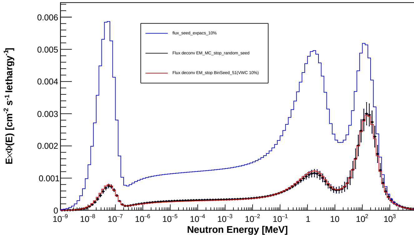
Spectrum_LCO_Event_8_timegrid_15_ndet_11_Random_Seed
