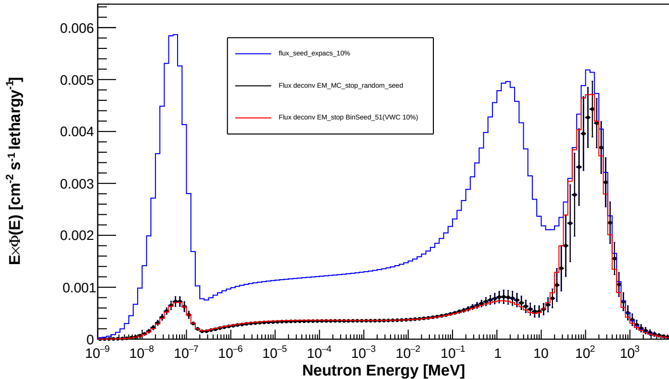
Spectrum_LCO_Event_1_timegrid_15_ndet_11_Random_Seed
