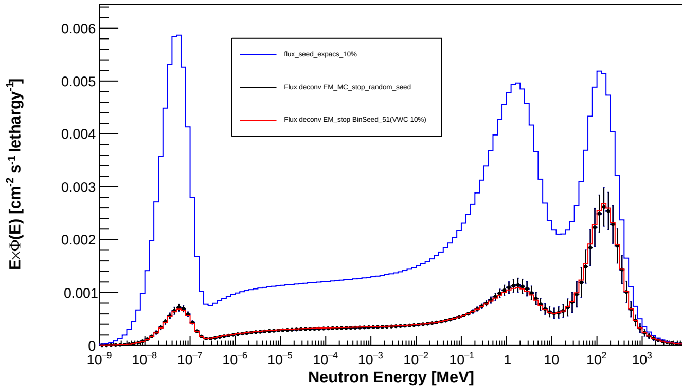
Spectrum_LCO_Event_15_timegrid_15_ndet_11_Random_Seed
