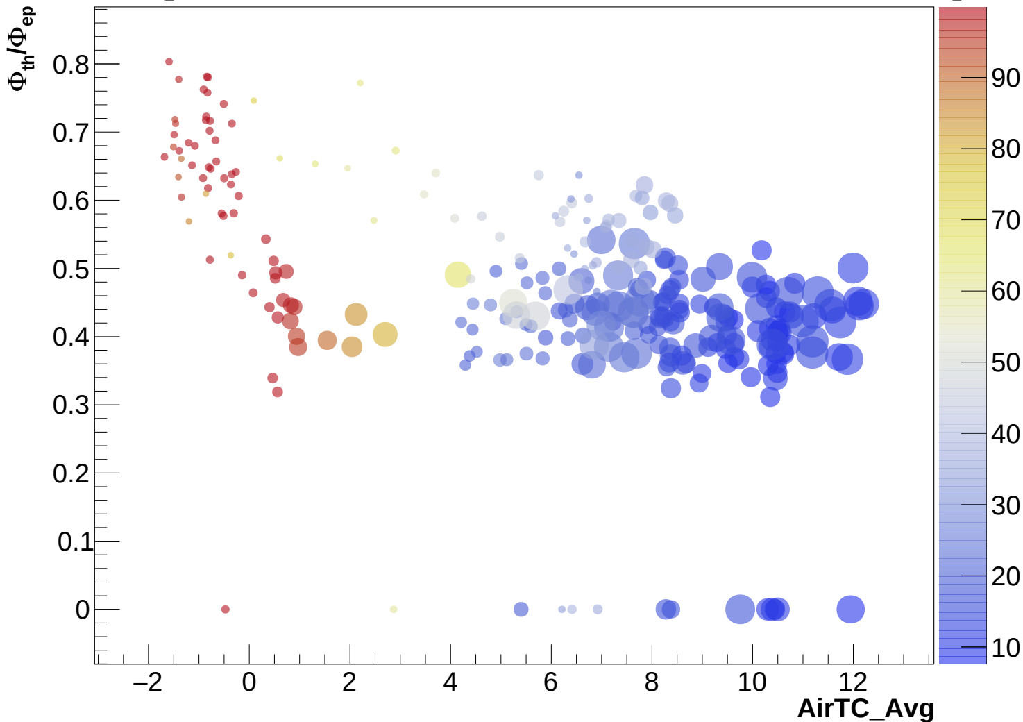
Scatter Plot 1: AirTC_Avg, \Phi_{th}/\Phi_{ep} , RH_Min, TC_5cm
