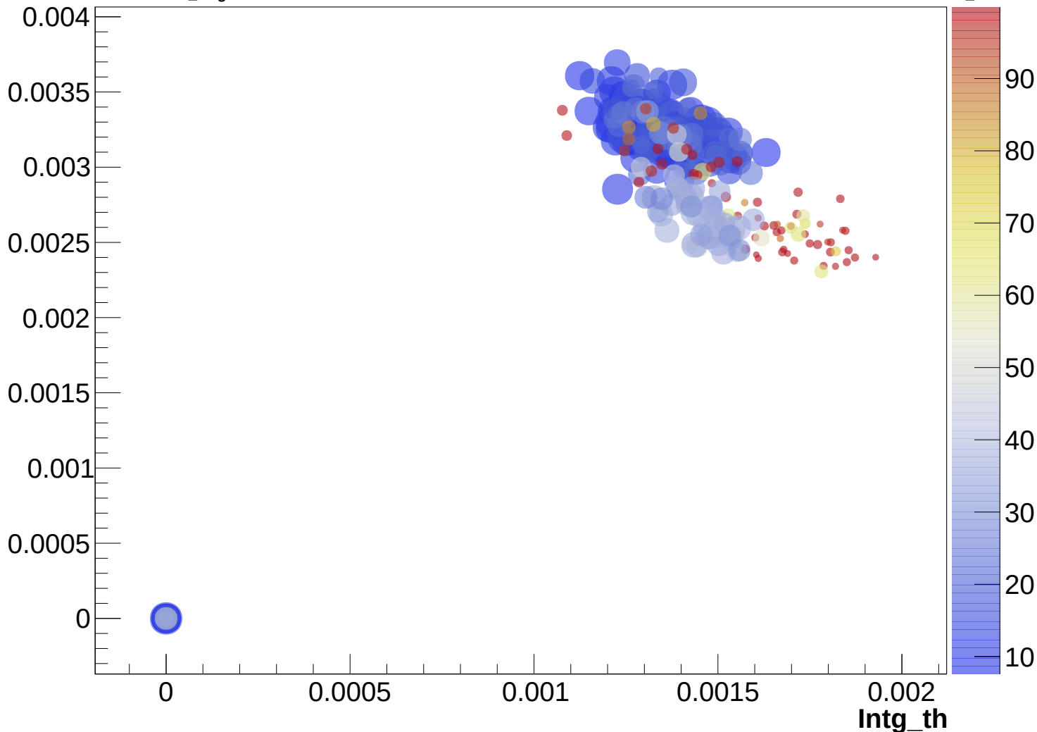
Scatter Plot 13: Intg_th, Intg_ep, RH_Min, AirTC_Avg
