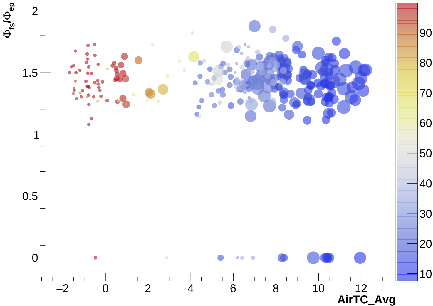
Scatter Plot 4: AirTC_Avg, \Phi_{fs}/\Phi_{ep} , RH_Min, TC_5cm
