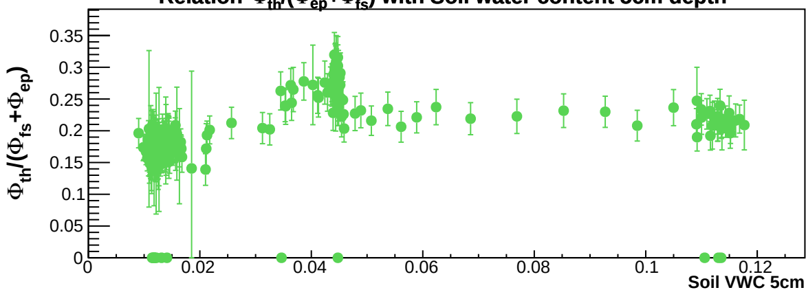
Relation \Phi_{th}/(\Phi_{ep}+\Phi_{fs}) with Soil water content 5cm depth
