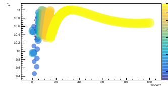
LCO_event_158_timegrid_15_ndet_11_scatterplot
