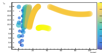
LCO_event_160_timegrid_15_ndet_11_scatterplot
