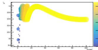
LCO_event_156_timegrid_15_ndet_11_scatterplot
