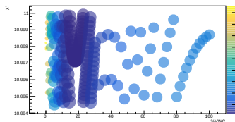
LCO_event_162_timegrid_15_ndet_11_scatterplot
