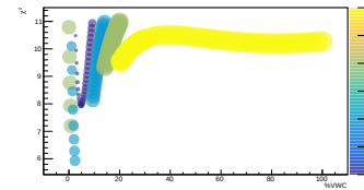
LCO_event_245_timegrid_15_ndet_11_scatterplot
