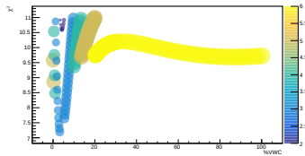
LCO_event_246_timegrid_15_ndet_11_scatterplot
