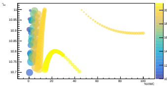
LCO_event_237_timegrid_15_ndet_11_scatterplot
