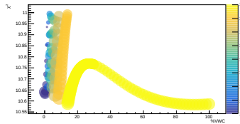
LCO_event_239_timegrid_15_ndet_11_scatterplot
