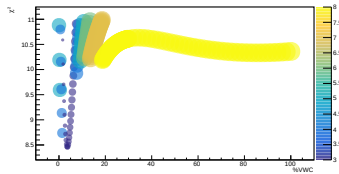
LCO_event_247_timegrid_15_ndet_11_scatterplot
