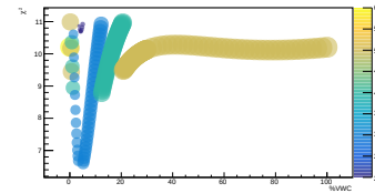
LCO_event_248_timegrid_15_ndet_11_scatterplot
