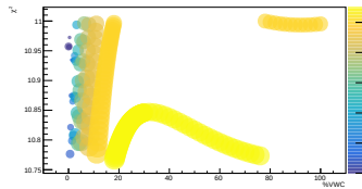
LCO_event_236_timegrid_15_ndet_11_scatterplot
