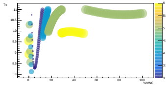
LCO_event_238_timegrid_15_ndet_11_scatterplot
