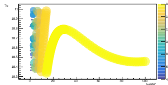
LCO_event_146_timegrid_15_ndet_11_scatterplot
