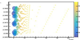
LCO_event_145_timegrid_15_ndet_11_scatterplot
