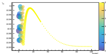
LCO_event_151_timegrid_15_ndet_11_scatterplot
