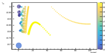
LCO_event_144_timegrid_15_ndet_11_scatterplot
