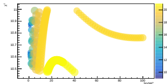
LCO_event_141_timegrid_15_ndet_11_scatterplot
