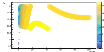
LCO_event_140_timegrid_15_ndet_11_scatterplot
