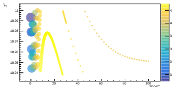
LCO_event_142_timegrid_15_ndet_11_scatterplot
