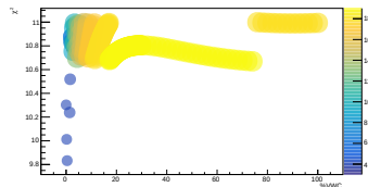
LCO_event_143_timegrid_15_ndet_11_scatterplot
