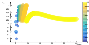
LCO_event_148_timegrid_15_ndet_11_scatterplot
