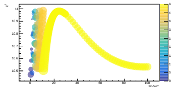
LCO_event_147_timegrid_15_ndet_11_scatterplot
