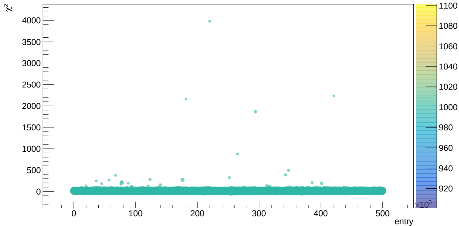
LCO_event_41_timegrid_15_ndet_11_scatterplot_MC_31006_it
