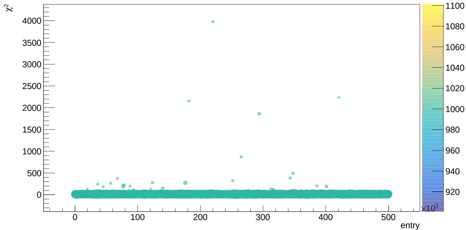
LCO_event_41_timegrid_15_ndet_11_scatterplot_MC_42043_it
