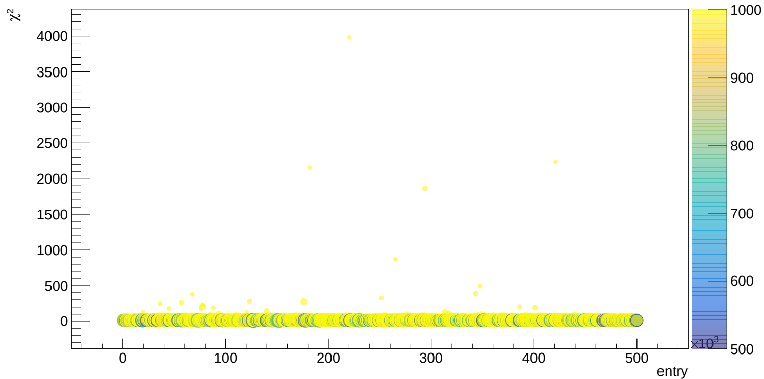
LCO_event_41_timegrid_15_ndet_11_scatterplot_MC_49526_it
