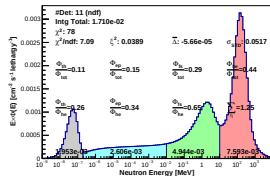
Spectrum_LCO_Event_41_Staps_7_BinSeed_105(WC 20.8%)
