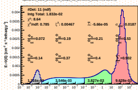
Spectrum_LCO_Event_41_Staps_19_BinSeed_105(WC 20.8%)
