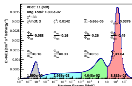
Spectrum_LCO_Event_41_Staps_11_BinSeed_105(WC 20.8%)
