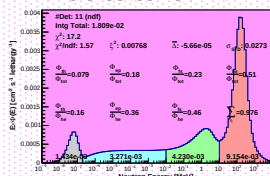
Spectrum_LCO_Event_41_Staps_16_BinSeed_105(WC 20.8%)
