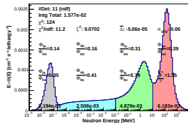
Spectrum_LCO_Event_41_Staps_6_BinSeed_105(WC 20.8%)
