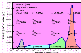
Spectrum_LCO_Event_41_Staps_14_BinSeed_105(WC 20.8%)
