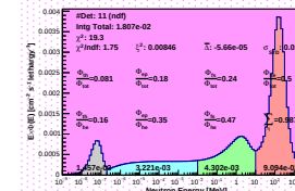
Spectrum_LCO_Event_41_Staps_15_BinSeed_105(WC 20.8%)
