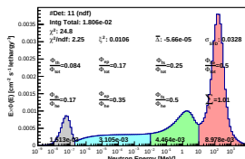
Spectrum_LCO_Event_41_Staps_13_BinSeed_105(WC 20.8%)
