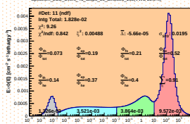
Spectrum_LCO_Event_41_Staps_18_BinSeed_105(WC 20.8%)
