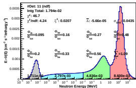
Spectrum_LCO_Event_41_Staps_9_BinSeed_105(WC 20.8%)
