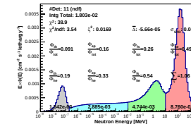
Spectrum_LCO_Event_41_Staps_10_BinSeed_105(WC 20.8%)
