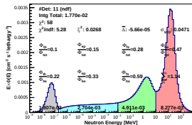
Spectrum_LCO_Event_41_Staps_8_BinSeed_105(WC 20.8%)
