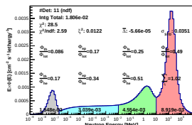
Spectrum_LCO_Event_41_Staps_12_BinSeed_105(WC 20.8%)
