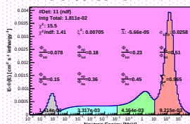
Spectrum_LCO_Event_41_Staps_17_BinSeed_105(WC 20.8%)
