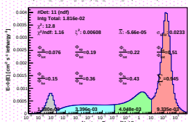
Spectrum_LCO_Event_41_Steps_19_BinSeed_107(WVC 21.2%)
