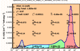
Spectrum_LCO_Event_41_Steps_17_BinSeed_107(WVC 21.2%)
