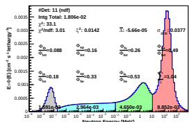
Spectrum_LCO_Event_41_Steps_11_BinSeed_107(WVC 21.2%)
