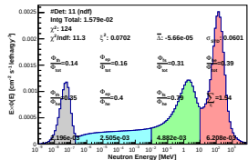
Spectrum_LCO_Event_41_Steps_6_BinSeed_107(WVC 21.2%)
