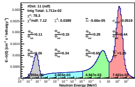
Spectrum_LCO_Event_41_Steps_7_BinSeed_107(WVC 21.2%)
