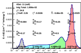
Spectrum_LCO_Event_41_Steps_13_BinSeed_107(WVC 21.2%)
