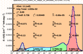
Spectrum_LCO_Event_41_Steps_20_BinSeed_107(WVC 21.2%)
