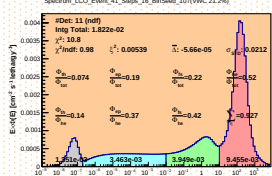
Spectrum_LCO_Event_41_Steps_16_BinSeed_107(WVC 21.2%)
