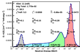
Spectrum_LCO_Event_41_Steps_8_BinSeed_107(WVC 21.2%)
