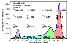
Spectrum_LCO_Event_41_Steps_9_BinSeed_107(WVC 21.2%)
