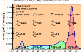
Spectrum_LCO_Event_41_Steps_18_BinSeed_107(WVC 21.2%)
