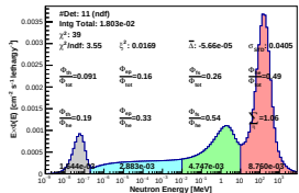
Spectrum_LCO_Event_41_Steps_10_BinSeed_107(WVC 21.2%)
