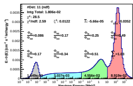
Spectrum_LCO_Event_41_Steps_12_BinSeed_107(WVC 21.2%)
