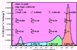
Spectrum_LCO_Event_41_Steps_14_BinSeed_107(WVC 21.2%)
