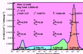
Spectrum_LCO_Event_41_Steps_16_BinSeed_112(WC 22.2%)
