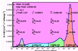
Spectrum_LCO_Event_41_Steps_20_BinSeed_112(WC 22.2%)
