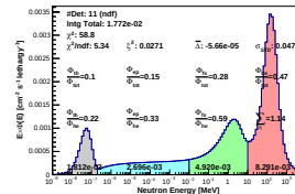
Spectrum_LCO_Event_41_Steps_8_BinSeed_112(WC 22.2%)
