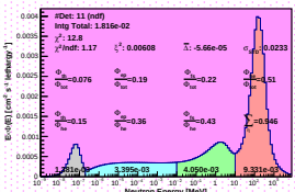
Spectrum_LCO_Event_41_Steps_19_BinSeed_112(WC 22.2%)
