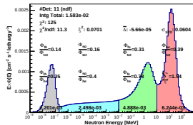
Spectrum_LCO_Event_41_Steps_6_BinSeed_112(WC 22.2%)
