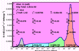
Spectrum_LCO_Event_41_Steps_17_BinSeed_112(WC 22.2%)
