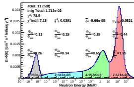
Spectrum_LCO_Event_41_Steps_7_BinSeed_112(WC 22.2%)
