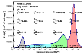
Spectrum_LCO_Event_41_Steps_10_BinSeed_112(WC 22.2%)
