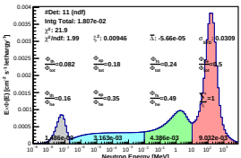
Spectrum_LCO_Event_41_Steps_14_BinSeed_112(WC 22.2%)
