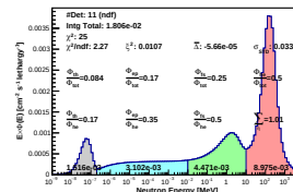
Spectrum_LCO_Event_41_Steps_13_BinSeed_112(WC 22.2%)
