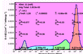
Spectrum_LCO_Event_41_Steps_18_BinSeed_112(WC 22.2%)
