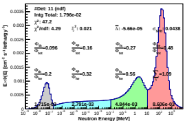
Spectrum_LCO_Event_41_Steps_9_BinSeed_112(WC 22.2%)
