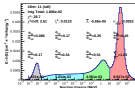
Spectrum_LCO_Event_41_Steps_12_BinSeed_112(WC 22.2%)
