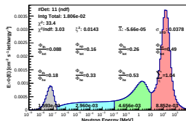
Spectrum_LCO_Event_41_Steps_11_BinSeed_112(WC 22.2%)
