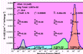
Spectrum_LCO_Event_41_Steps_15_BinSeed_112(WC 22.2%)
