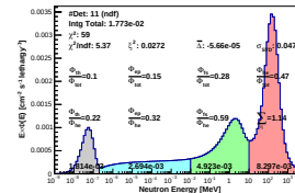
Spectrum_LCO_Event_41_Staps_8_BinSd_115(WVC 22.8%)
