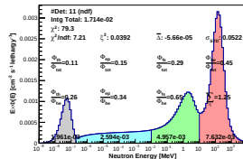
Spectrum_LCO_Event_41_Staps_7_BinSd_115(WVC 22.8%)
