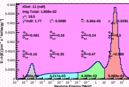
Spectrum_LCO_Event_41_Staps_15_BinSd_115(WVC 22.8%)
