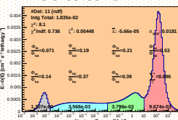
Spectrum_LCO_Event_41_Staps_20_BinSd_115(WVC 22.8%)
