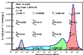
Spectrum_LCO_Event_41_Staps_14_BinSd_115(WVC 22.8%)
