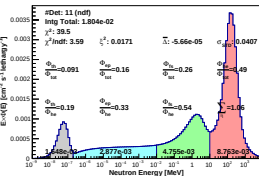
Spectrum_LCO_Event_41_Staps_10_BinSd_115(WVC 22.8%)
