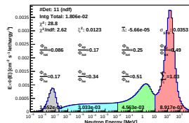
Spectrum_LCO_Event_41_Staps_12_BinSd_115(WVC 22.8%)
