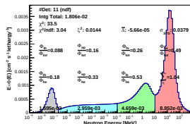
Spectrum_LCO_Event_41_Staps_11_BinSd_115(WVC 22.8%)
