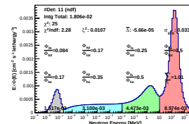
Spectrum_LCO_Event_41_Staps_13_BinSd_115(WVC 22.8%)
