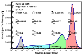
Spectrum_LCO_Event_41_Staps_9_BinSd_115(WVC 22.8%)
