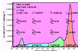
Spectrum_LCO_Event_41_Staps_17_BinSd_115(WVC 22.8%)
