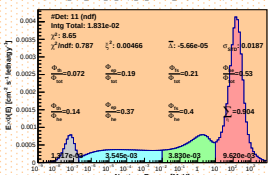
Spectrum_LCO_Event_41_Staps_19_BinSd_115(WVC 22.8%)
