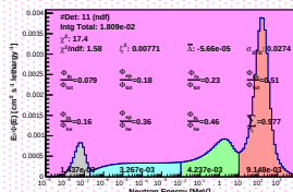
Spectrum_LCO_Event_41_Staps_16_BinSd_115(WVC 22.8%)
