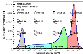
Spectrum_LCO_Event_41_Staps_6_BinSd_115(WVC 22.8%)
