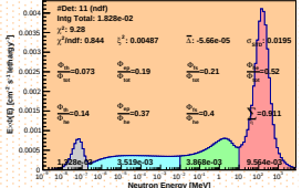
Spectrum_LCO_Event_41_Steps_18_BinSeed_116(WVC 23%)
