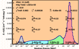
Spectrum_LCO_Event_41_Steps_16_BinSeed_116(WVC 23%)
