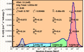
Spectrum_LCO_Event_41_Steps_19_BinSeed_116(WVC 23%)
