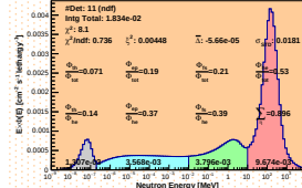
Spectrum_LCO_Event_41_Steps_20_BinSeed_116(WVC 23%)
