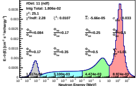
Spectrum_LCO_Event_41_Steps_13_BinSeed_116(WVC 23%)
