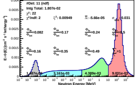
Spectrum_LCO_Event_41_Steps_14_BinSeed_116(WVC 23%)
