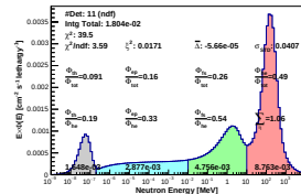
Spectrum_LCO_Event_41_Steps_10_BinSeed_116(WVC 23%)
