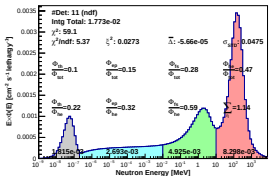
Spectrum_LCO_Event_41_Steps_8_BinSeed_116(WVC 23%)
