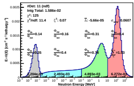
Spectrum_LCO_Event_41_Steps_6_BinSeed_116(WVC 23%)
