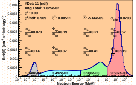
Spectrum_LCO_Event_41_Steps_17_BinSeed_116(WVC 23%)
