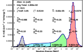
Spectrum_LCO_Event_41_Steps_11_BinSeed_116(WVC 23%)
