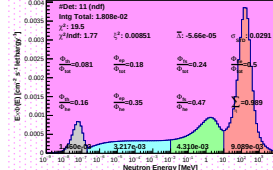
Spectrum_LCO_Event_41_Steps_15_BinSeed_116(WVC 23%)
