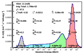
Spectrum_LCO_Event_41_Steps_9_BinSeed_116(WVC 23%)
