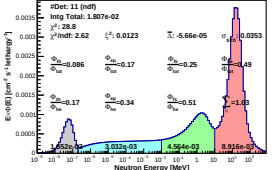
Spectrum_LCO_Event_41_Steps_12_BinSeed_116(WVC 23%)
