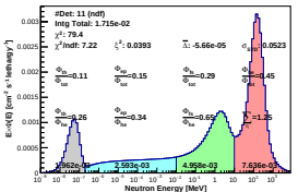
Spectrum_LCO_Event_41_Steps_7_BinSeed_116(WVC 23%)
