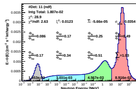
Spectrum_LCO_Event_41_Steps_12BisSeed_119(WVC 23.6%)
