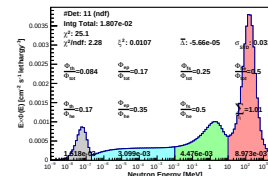
Spectrum_LCO_Event_41_Steps_13BisSeed_119(WVC 23.6%)
