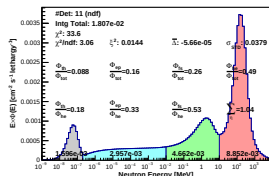
Spectrum_LCO_Event_41_Steps_11BisSeed_119(WVC 23.6%)
