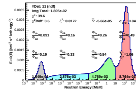
Spectrum_LCO_Event_41_Steps_10BisSeed_119(WVC 23.6%)
