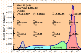
Spectrum_LCO_Event_41_Steps_19BisSeed_119(WVC 23.6%)
