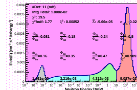
Spectrum_LCO_Event_41_Steps_15BisSeed_119(WVC 23.6%)
