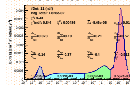
Spectrum_LCO_Event_41_Steps_18BisSeed_119(WVC 23.6%)
