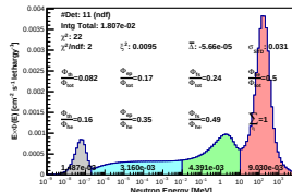
Spectrum_LCO_Event_41_Steps_14BisSeed_119(WVC 23.6%)
