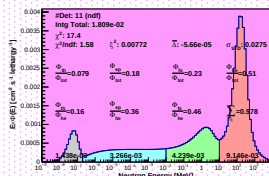
Spectrum_LCO_Event_41_Steps_16BisSeed_119(WVC 23.6%)
