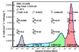
Spectrum_LCO_Event_41_Steps_9BisSeed_119(WVC 23.6%)
