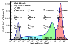
Spectrum_LCO_Event_41_Steps_6BisSeed_119(WVC 23.6%)
