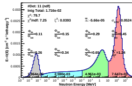
Spectrum_LCO_Event_41_Steps_7BisSeed_119(WVC 23.6%)
