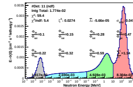
Spectrum_LCO_Event_41_Steps_8BisSeed_119(WVC 23.6%)
