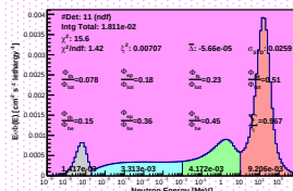
Spectrum_LCO_Event_41_Steps_17BisSeed_119(WVC 23.6%)
