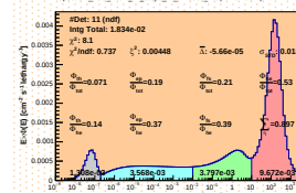
Spectrum_LCO_Event_41_Steps_20BisSeed_119(WVC 23.6%)
