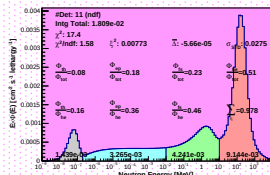
Spectrum_LCO_Event_41_Staps_16_BinSeed_125(WC 24.8%)
