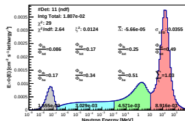
Spectrum_LCO_Event_41_Staps_12_BinSeed_125(WC 24.8%)
