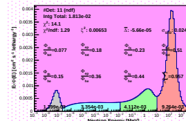
Spectrum_LCO_Event_41_Staps_18_BinSeed_125(WC 24.8%)
