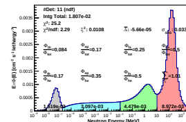
Spectrum_LCO_Event_41_Staps_13_BinSeed_125(WC 24.8%)
