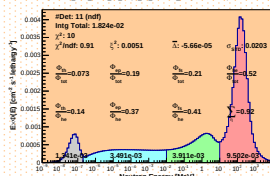
Spectrum_LCO_Event_41_Staps_17_BinSeed_125(WC 24.8%)
