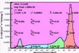
Spectrum_LCO_Event_41_Staps_15_BinSeed_125(WC 24.8%)
