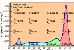
Spectrum_LCO_Event_41_Staps_20_BinSeed_125(WC 24.8%)
