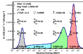
Spectrum_LCO_Event_41_Staps_6_BinSeed_125(WC 24.8%)
