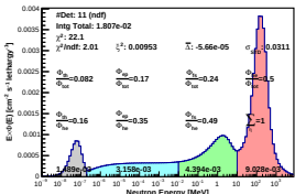
Spectrum_LCO_Event_41_Staps_14_BinSeed_125(WC 24.8%)
