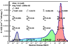
Spectrum_LCO_Event_41_Staps_10_BinSeed_125(WC 24.8%)
