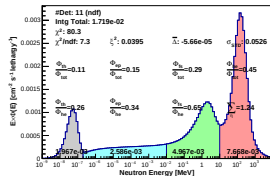
Spectrum_LCO_Event_41_Staps_7_BinSeed_125(WC 24.8%)
