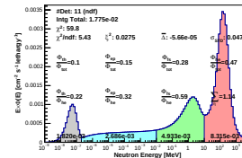
Spectrum_LCO_Event_41_Staps_8_BinSeed_125(WC 24.8%)
