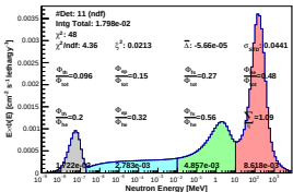
Spectrum_LCO_Event_41_Staps_9_BinSeed_125(WC 24.8%)
