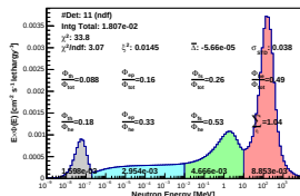
Spectrum_LCO_Event_41_Staps_11_BinSeed_125(WC 24.8%)
