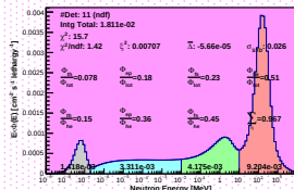
Spectrum_LCO_Event_41_Steps_17_BinSeed_127(WVC 25.2%)
