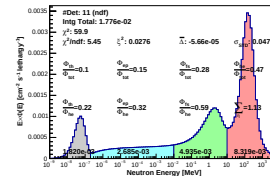
Spectrum_LCO_Event_41_Steps_8_BinSeed_127(WVC 25.2%)
