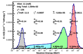
Spectrum_LCO_Event_41_Steps_6_BinSeed_127(WVC 25.2%)
