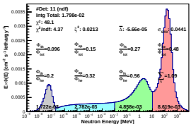
Spectrum_LCO_Event_41_Steps_9_BinSeed_127(WVC 25.2%)
