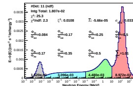
Spectrum_LCO_Event_41_Steps_13_BinSeed_127(WVC 25.2%)
