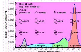
Spectrum_LCO_Event_41_Steps_18_BinSeed_127(WVC 25.2%)
