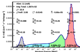
Spectrum_LCO_Event_41_Steps_11_BinSeed_127(WVC 25.2%)
