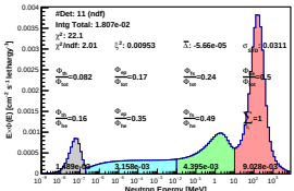
Spectrum_LCO_Event_41_Steps_14_BinSeed_127(WVC 25.2%)
