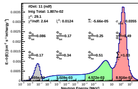
Spectrum_LCO_Event_41_Steps_12_BinSeed_127(WVC 25.2%)
