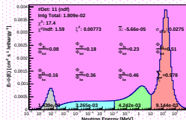
Spectrum_LCO_Event_41_Steps_16_BinSeed_127(WVC 25.2%)
