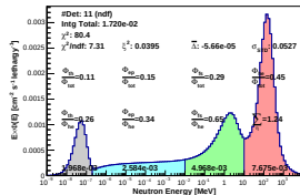
Spectrum_LCO_Event_41_Steps_7_BinSeed_127(WVC 25.2%)
