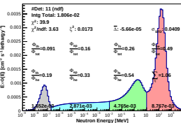
Spectrum_LCO_Event_41_Steps_10_BinSeed_127(WVC 25.2%)
