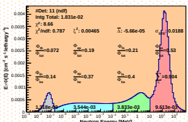
Spectrum_LCO_Event_41_Steps_19_BinSeed_127(WVC 25.2%)
