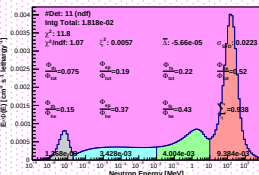
Spectrum_LCO_Event_41_Steps_20_BinSeed_127(WVC 25.2%)
