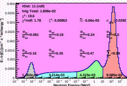
Spectrum_LCO_Event_41_Steps_15_BinSeed_127(WVC 25.2%)
