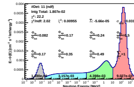
Spectrum_LCO_Event_41_Staps_14_BinSeed_134(WVC 26.6%)
