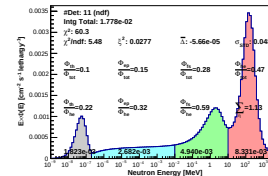
Spectrum_LCO_Event_41_Staps_8_BinSeed_134(WVC 26.6%)
