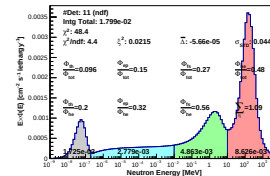
Spectrum_LCO_Event_41_Staps_9_BinSeed_134(WVC 26.6%)
