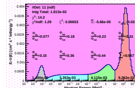
Spectrum_LCO_Event_41_Staps_18_BinSeed_134(WVC 26.6%)
