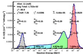
Spectrum_LCO_Event_41_Staps_7_BinSeed_134(WVC 26.6%)
