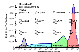
Spectrum_LCO_Event_41_Staps_13_BinSeed_134(WVC 26.6%)
