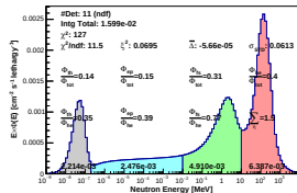
Spectrum_LCO_Event_41_Staps_6_BinSeed_134(WVC 26.6%)
