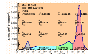
Spectrum_LCO_Event_41_Staps_20_BinSeed_134(WVC 26.6%)
