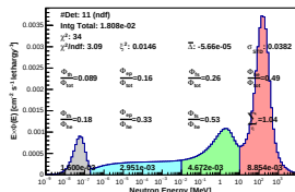
Spectrum_LCO_Event_41_Staps_11_BinSeed_134(WVC 26.6%)
