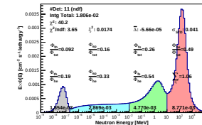
Spectrum_LCO_Event_41_Staps_10_BinSeed_134(WVC 26.6%)
