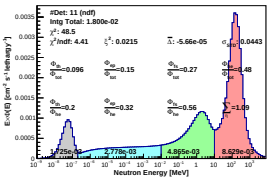
Spectrum_LCO_Event_41_Steps_9_BinSeed_137(WVC 27.2%)
