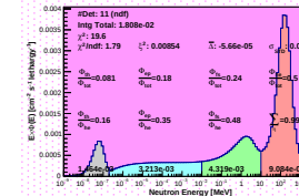
Spectrum_LCO_Event_41_Steps_15_BinSeed_137(WVC 27.2%)
