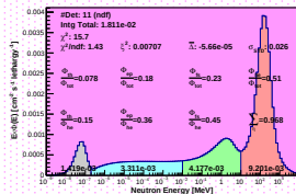
Spectrum_LCO_Event_41_Steps_17_BinSeed_137(WVC 27.2%)
