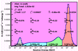
Spectrum_LCO_Event_41_Steps_19_BinSeed_137(WVC 27.2%)
