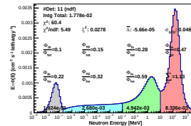
Spectrum_LCO_Event_41_Steps_8_BinSeed_137(WVC 27.2%)
