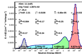
Spectrum_LCO_Event_41_Steps_13_BinSeed_137(WVC 27.2%)
