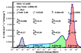
Spectrum_LCO_Event_41_Steps_12_BinSeed_137(WVC 27.2%)
