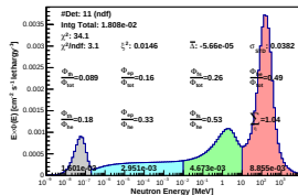
Spectrum_LCO_Event_41_Steps_11_BinSeed_137(WVC 27.2%)
