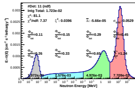
Spectrum_LCO_Event_41_Steps_7_BinSeed_137(WVC 27.2%)
