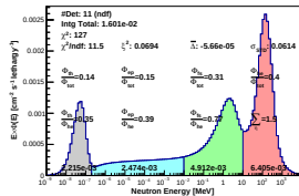
Spectrum_LCO_Event_41_Steps_6_BinSeed_137(WVC 27.2%)
