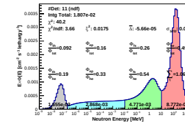
Spectrum_LCO_Event_41_Steps_10_BinSeed_137(WVC 27.2%)
