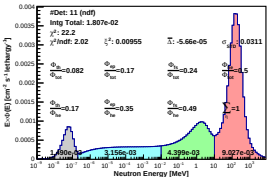
Spectrum_LCO_Event_41_Steps_14_BinSeed_137(WVC 27.2%)
