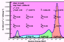
Spectrum_LCO_Event_41_Steps_16_BinSeed_137(WVC 27.2%)
