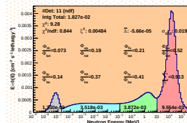
Spectrum_LCO_Event_41_Steps_18_BinSeed_137(WVC 27.2%)
