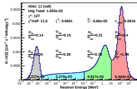
Spectrum_LCO_Event_41_Steps_6_BinSeed_144(WC 28.6%)
