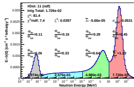
Spectrum_LCO_Event_41_Steps_7_BinSeed_144(WC 28.6%)
