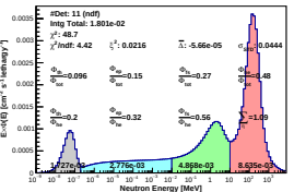
Spectrum_LCO_Event_41_Steps_9_BinSeed_144(WC 28.6%)
