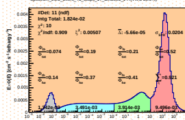
Spectrum_LCO_Event_41_Steps_17_BinSeed_144(WC 28.6%)
