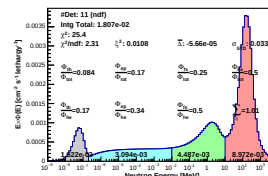
Spectrum_LCO_Event_41_Steps_13_BinSeed_144(WC 28.6%)
