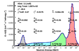
Spectrum_LCO_Event_41_Steps_10_BinSeed_144(WC 28.6%)
