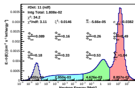
Spectrum_LCO_Event_41_Steps_11_BinSeed_144(WC 28.6%)
