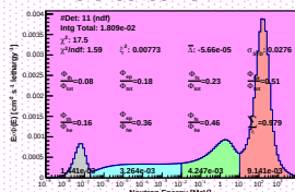
Spectrum_LCO_Event_41_Steps_16_BinSeed_144(WC 28.6%)
