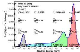
Spectrum_LCO_Event_41_Steps_8_BinSeed_144(WC 28.6%)
