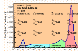
Spectrum_LCO_Event_41_Steps_20_BinSeed_144(WC 28.6%)
