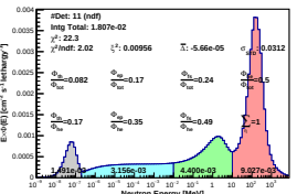
Spectrum_LCO_Event_41_Steps_14_BinSeed_144(WC 28.6%)
