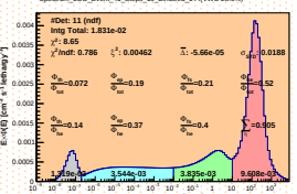
Spectrum_LCO_Event_41_Steps_19_BinSeed_144(WC 28.6%)
