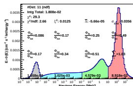
Spectrum_LCO_Event_41_Steps_12_BinSeed_144(WC 28.6%)
