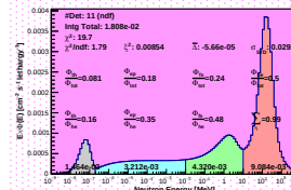
Spectrum_LCO_Event_41_Steps_15_BinSeed_144(WC 28.6%)
