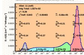
Spectrum_LCO_Event_41_Steps_18_BinSeed_144(WC 28.6%)
